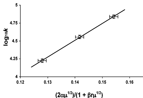
Figure 6. Extended Debye–Hückel equation plot of rate constants for electron transfer from 1_{\text{red}} to 2_{\text{red}} ; R^2 = 0.9997 , the slope gives a charge product, z_1z_2 , of 23 \pm 1 , and extrapolation to zero ionic strength ( \mu = 0 ) gives k_0 = 17 \pm 2 \text{ M}^{-1} \text{ s}^{-1} . Changes in ionic strength during the reaction—because of changes in the charges of the reacting species—were small relative to the total ionic strength and relative to the statistical uncertainty involved in extrapolation to \mu = 0 .
