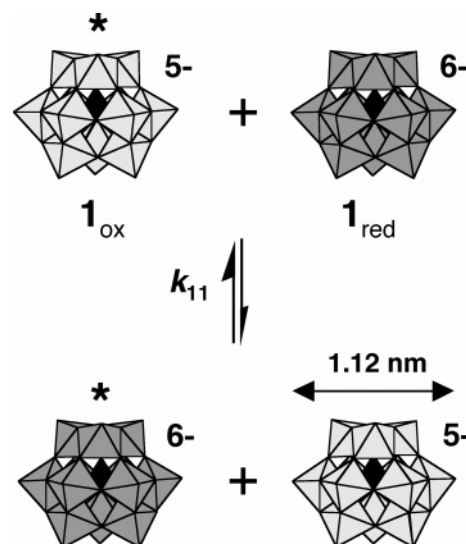
Figure 1. Electron exchange between \alpha\text{-AlW}_{12}\text{O}_{40}^{5-} ( 1 ox ) and \alpha\text{-AlW}_{12}\text{O}_{40}^{6-} ( 1 red ). The \alpha -Keggin anions, shown in coordination-polyhedron notation, are 1.12 nm in diameter and possess tetrahedral ( T_d ) symmetry. In each anion, 12 W addendum atoms are at the center of \text{WO}_6 polyhedra, which each possess C_{4v} symmetry and have O atoms at their vertices. At the center of each cluster (shaded) is a tetrahedral aluminate oxoanion, \text{Al}^{\text{III}}\text{O}_4^{5-} .
