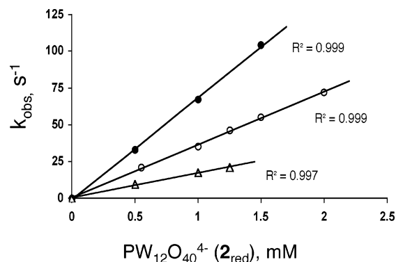
Figure 5. Rate constants, k_{\text{obs}} , for the oxidation \alpha\text{-AlW}_{12}\text{O}_{40}^{6-} ( 1_{\text{red}} ; limiting reagent) by \alpha\text{-PW}_{12}\text{O}_{40}^{4-} ( 2_{\text{red}} ; present at large molar excess) at three initial ionic strength values ( \mu , adjusted by addition of NaCl), 65 (▲), 97 (○), and 140 (●) mM, in 50 mM phosphate buffer (pH 2.15) at 25 °C. The points at the origin are for [2_{\text{red}}] = 0 mM, at which no reaction occurs ( k_{\text{obs}} = 0 s -1 ).
