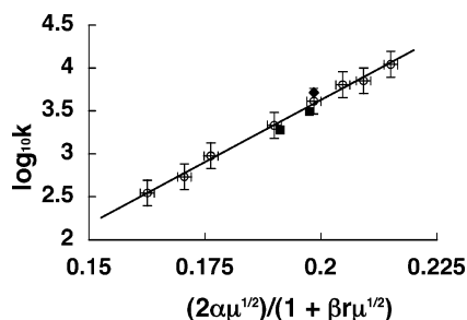
Figure 4. Plot of \log k for electron self-exchange between 1_{\text{ox}} and 1_{\text{red}} as a function of ionic strength, \mu . From the extended Debye–Hückel equation, \log k = \log k_0 + 2z_1z_2\alpha\mu^{1/2}/(1 + \beta r\mu^{1/2}) ( \alpha = 0.509 , \beta = 0.33 \times 10^8 cm, and r is the hard-sphere collision distance, 1.12 nm); the slope ( R^2 = 0.996 ) gives the charge product, z_1z_2 , and the y intercept (at \mu = 0 ) gives k_{11} . Rate constants were obtained using total heteropolyanion concentrations, [\text{POM}]_{\text{total}} , of 4.6 mM at pH 7.2 (O) and pH 2.15 (◆); two rate constants (■) were obtained at pH 7.2, but with [\text{POM}]_{\text{total}} = 9.2 mM. Uncertainties (shown as error bars here) in k_{11} and in z_1z_2 (reported in the text) are 95% confidence intervals.
