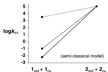
Figure 7. Zero-ionic-strength self-exchange rate constants for electron transfer between \alpha\text{-AlW}_{12}\text{O}_{40}^{6-} and \alpha\text{-AlW}_{12}\text{O}_{40}^{5-} ( 1_{\text{red}} and 1_{\text{ox}} ) and between \alpha\text{-PW}_{12}\text{O}_{40}^{4-} and \alpha\text{-PW}_{12}\text{O}_{40}^{3-} ( 2_{\text{red}} and 2_{\text{ox}} ). The rate constant for self-exchange between 2_{\text{red}} and 2_{\text{ox}} is at the upper right ( k_{11} = 1.1 \times 10^5 \text{ M}^{-1} \text{ s}^{-1} ; \log k_{11} = 5.04 ), and that for self-exchange between 1_{\text{red}} and 1_{\text{ox}} is at the lower left ( k_{11} = 6.5 \times 10^{-3} \text{ M}^{-1} \text{ s}^{-1} ; \log k_{11} = -2.19 ). See the text for descriptions of the three lines shown.
