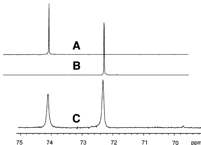
Figure 2. 27 Al NMR spectra of \alpha -AlW 12 O 40 6- ( 1 red , A), \alpha -AlW 12 O 40 5- ( 1 ox , B), and a mixture containing a 1.0:0.85 molar ratio of 1 ox to 1 red (C). The total concentration of POM anions present ( 1 ox + 1 red ) was 4.6 mM; [NaCl] was 0.68 M at pH 7.2 and 19.2 \pm 0.5 °C.
