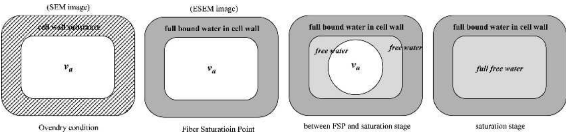
FIG. 4. Single cell structure change from dry to fully saturated condition.
