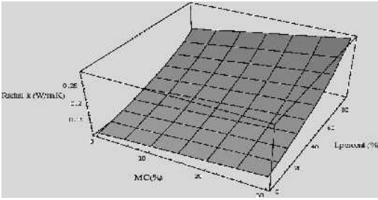
FIG. 7. Model-predicted radial thermal conductivity values for latewood percentages from 10% to 99% and MC from 0% to 30%.
