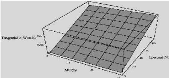
FIG. 6. Model-predicted tangential thermal conductivity values for latewood percentages from 10% to 99% and MC from 0% to 30%.
