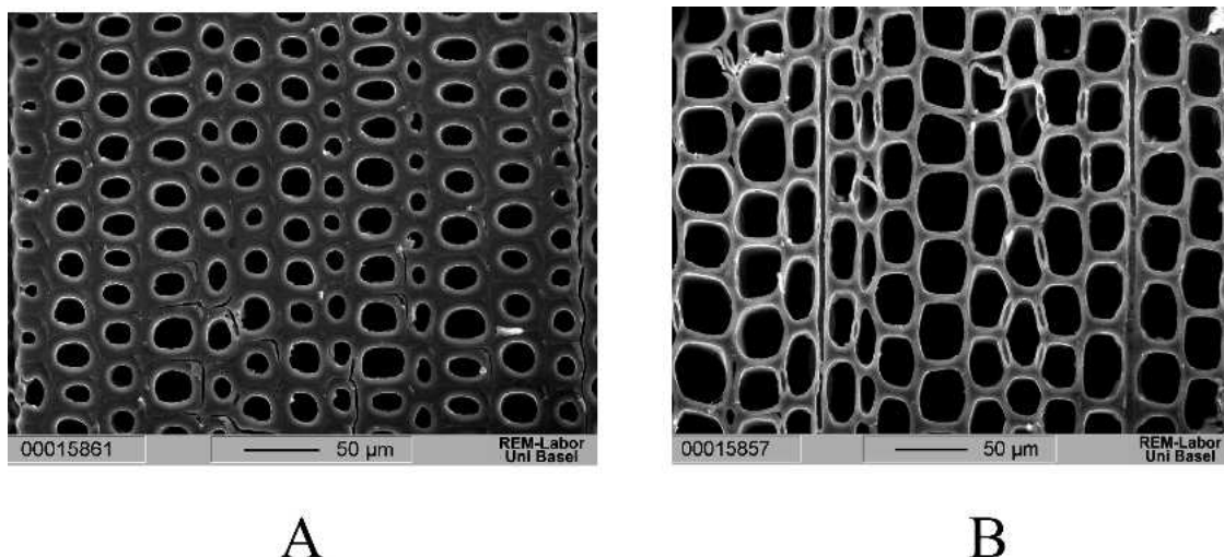
Fig. 2. Scots pine images, wet condition. A-latewood, B-earlywood.
