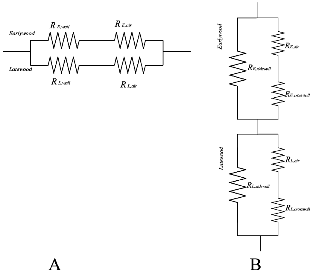
FIG. 5. Thermal resistance model for softwood species. A-tangential direction, B-radial direction.
