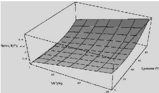
FIG. 8. Model-predicted ratio of radial versus tangential thermal conductivity values.
