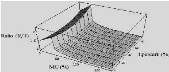
FIG. 11. Ratio of radial versus tangential thermal conductivity values predicted for Scots pine.
