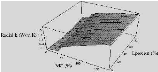
FIG. 10. Radial thermal conductivity values predicted for Scots pine for latewood percentage from 5% to 99% and MC from 0% to maximum 178%.
