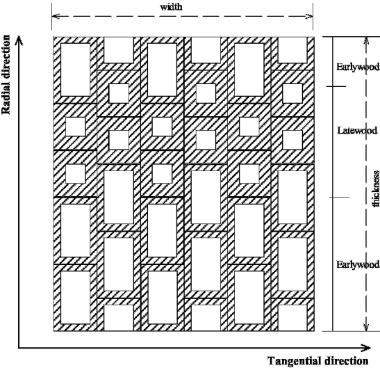
FIG. 3. Simplified structure model for softwoods.
