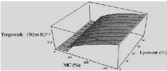
FIG. 9. Tangential thermal conductivity values predicted for Scots pine for latewood percentage from 5% to 99% and MC from 0% to maximum 178%.
