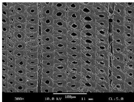
FIG. 1. Southern yellow pine images. A-latewood, B-earlywood.
