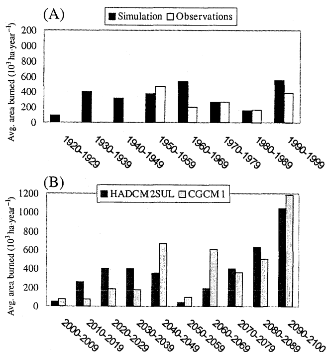
Fig. 8. Simulated annual average area burned by decade across the entire state of Alaska (A) under historical conditions (1922–1996) as compared with the decadal averages from the Alaska large-fire database (between 1950 and 1987, only fires >400 ha were reported; between 1988 and 2003, only fires >40 ha were reported) and (B) under HADCM2SUL and CGCM1 climate change scenarios.
