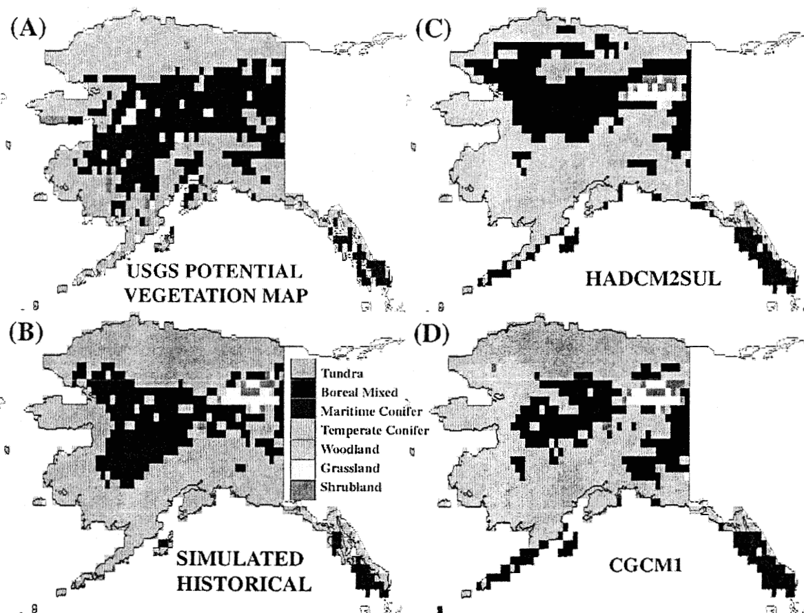
Fig. 5. Percent cover of the various vegetation types simulated across the state of Alaska under historical climate conditions (1922–1996) and under two climate change scenarios (HADCM2SUL and CGCM1).
