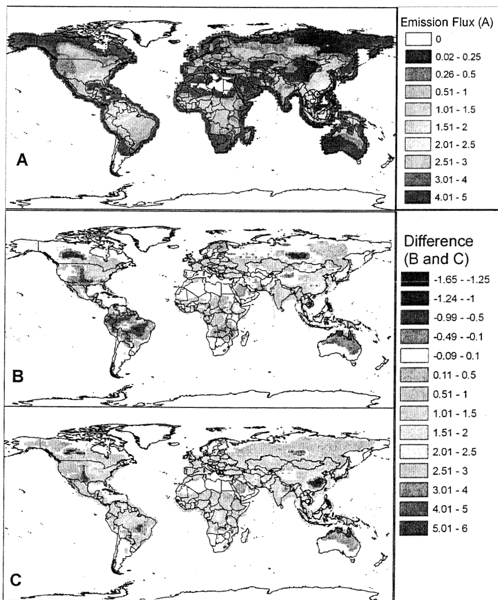
Figure 1. (a) Estimated isoprene emissions ( \text{mg isoprene m}^{-2} \text{ h}^{-1} ) for the BASE case. (b) Difference in isoprene emissions for ((FUTVEG-CURCLIM) - BASE). (c) Difference in isoprene emissions for ((FUTVEG-FUTCLIM) - BASE). All emissions shown ( \text{mg isoprene m}^{-2} \text{ h}^{-1} ) have been averaged for the month of July.
