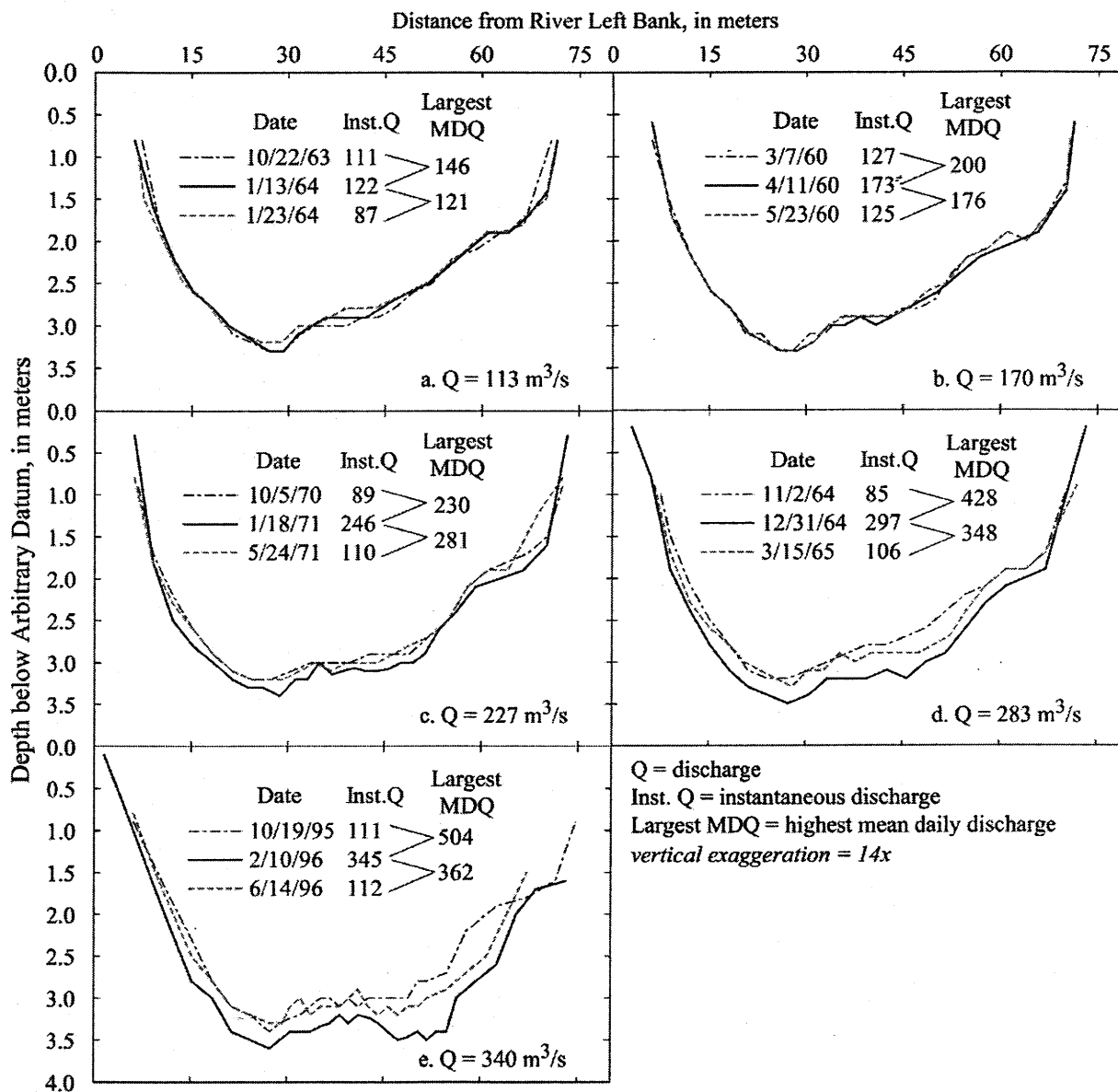
Figure 17. Cross-sectional profiles at the USGS measurement cross-section for the Deschutes River near Madras gage showing degree of bed response for flow events of different sizes.
