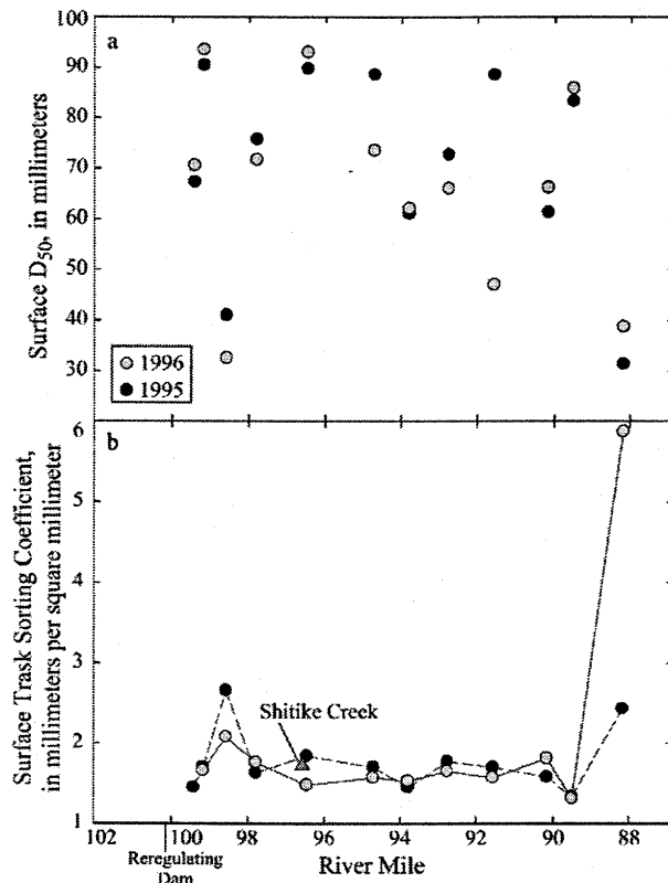
Figure 19. Grain-size data for bar and island heads in the primary study reach in 1995 and 1996: (a) Surface D_{50} values; (b) Task sorting coefficients for surface bed-material.
