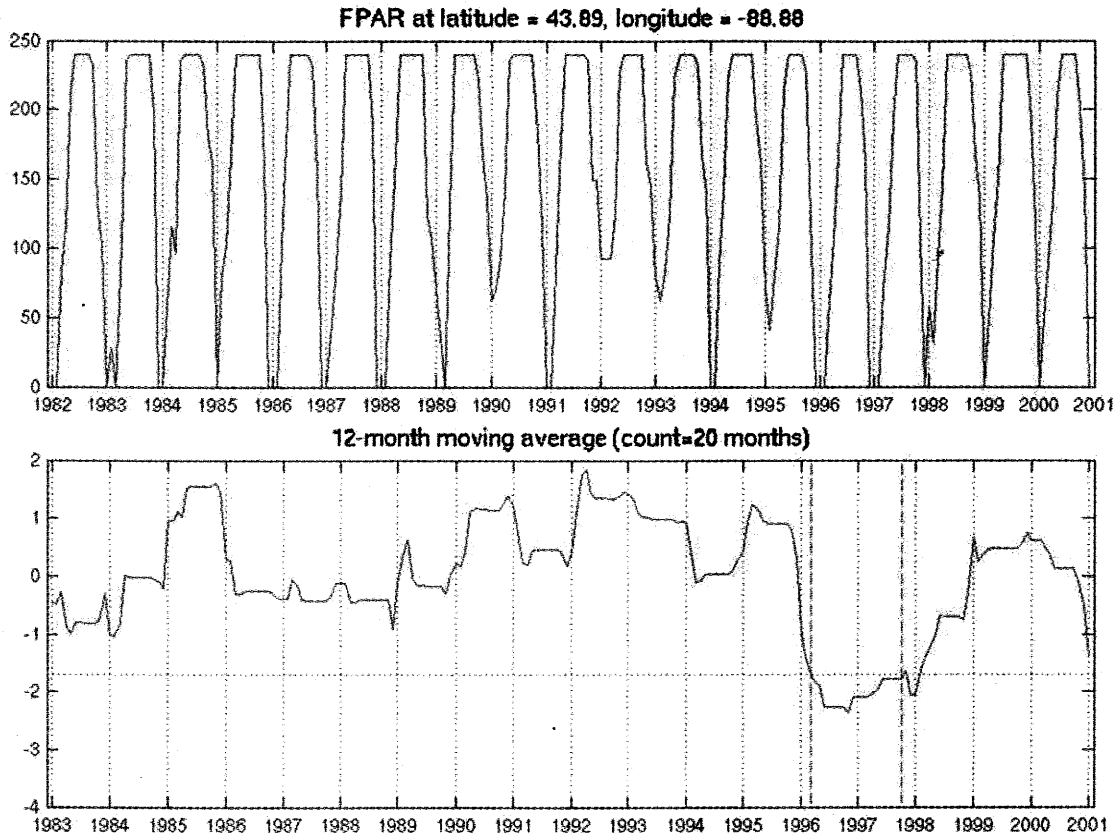
Figure 8. FPAR-LO event in Wisconsin 1996–1997, showing 2 consecutive years of winter-spring cold wave impacts on midwestern U.S. greenness profiles.
