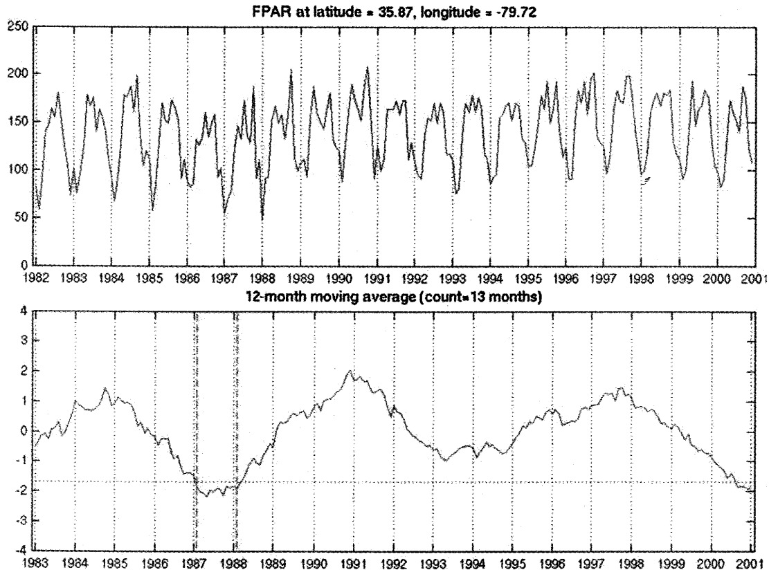
Figure 6. FPAR-LO event in North Carolina 1986, showing drought and heat wave impacts on southeastern U.S. greenness profiles.
