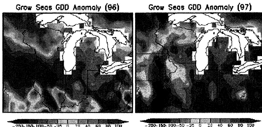
Figure 9. Anomalies in growing season (defined as the time period from the last spring freeze to the first fall freeze, inclusive, using 0°C as a temperature threshold) growing degree days (GDD, base 8°C) for 1996 (left) and 1997 (right).
