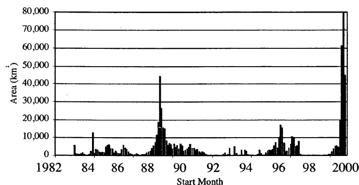
Figure 4. Distribution according to start month of land area detected with at least one FPAR-LO event in the time series 1982–2000.
