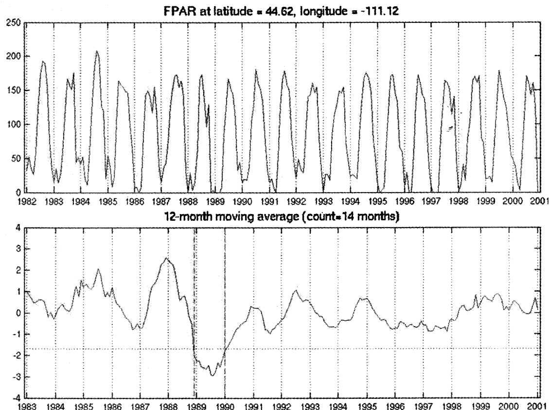
Figure 7. FPAR-LO event in the summer of 1988, centered several kilometres south of West Yellowstone, Montana at the North Fork Fire locations spreading from Yellowstone National Park.
