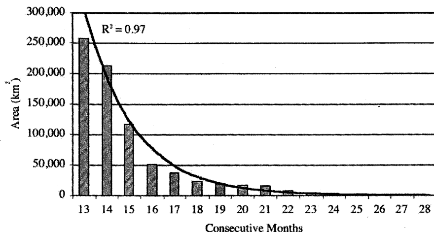
Figure 3. Distribution according to consecutive monthly time steps of land area detected with at least one FPAR-LO event in the time series 1982–2000.
