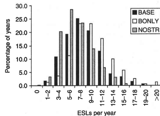
Fig. 4. Relative frequency histograms of number of exceeded simulation limit (ESL) fires per year on the Nevada-Yuba-Placer Ranger Unit, for the base-case (BASE), Schedule B only (BONLY) simulation, and the no structure protection (NOSTR) simulation.
