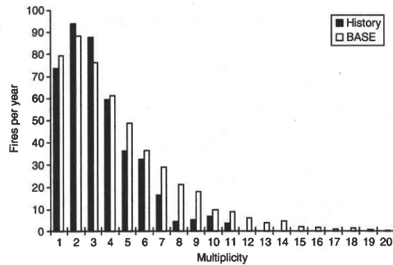
Fig. 5. Multiplicity for all fires in the historical period 1986–1994 and the base-case (BASE) simulation.
