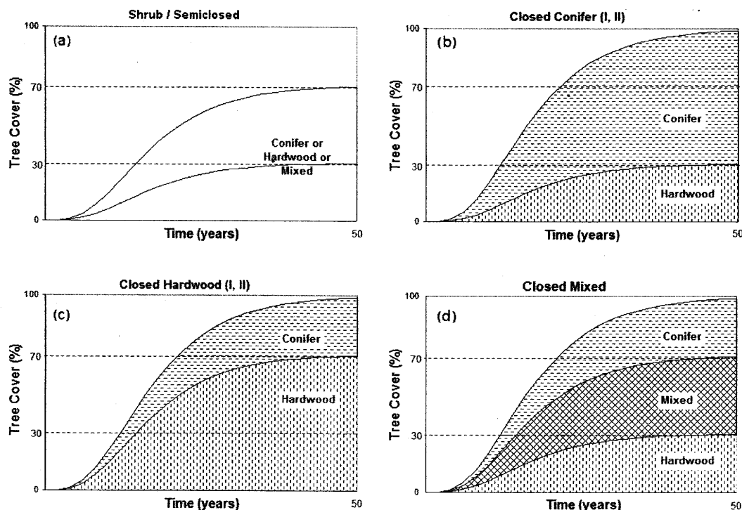
Fig. 2. Boundary conditions for successional trajectory categories. (a) Shrub trajectory has tree cover under 30%, and semiclosed trajectory has tree cover under 70%; (b) total tree cover is at least 70%, and conifer is dominant life form; (c) total tree cover is at least 70%, and hardwood is the dominant life form; (d) total tree cover is at least 70%, and conifer and hardwood are the co-dominant life forms.
