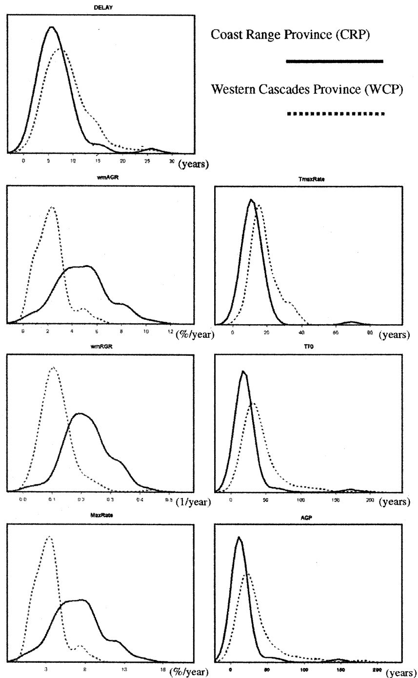
Fig. 8. Distribution of successional rate parameters.
