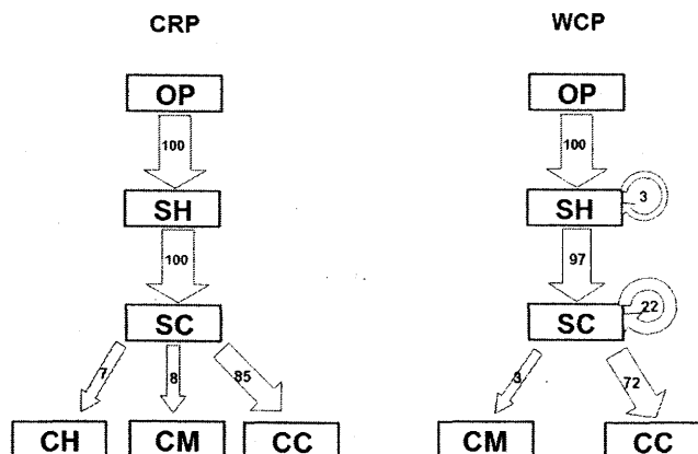
Fig. 7. Successional stage transition for the Coast Range Province (left) and the Western Cascades Province (right).
