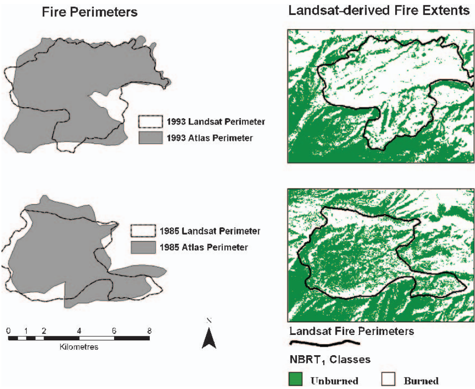
Figure 3. Comparison of 1985 and 1993 fire perimeters derived from fire atlas data and hand-digitized from Landsat TM imagery.
