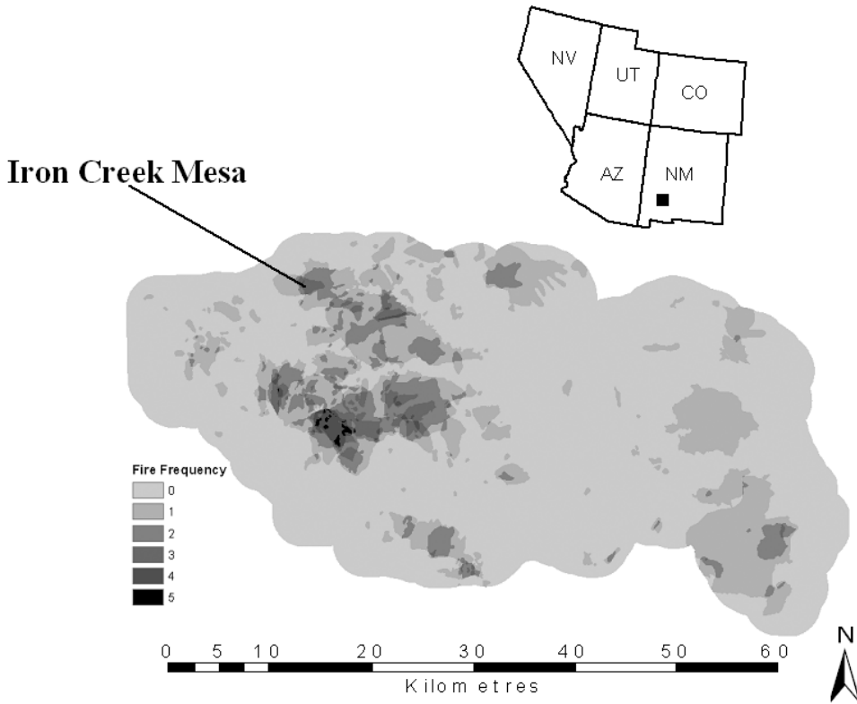
Figure 1. Study area within the Gila–Aldo Leopold Wilderness fire atlas.
