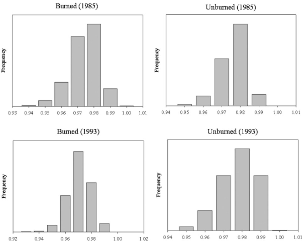
Figure 2. Histograms of NBRT index image region of interest data for assessment of normality.
