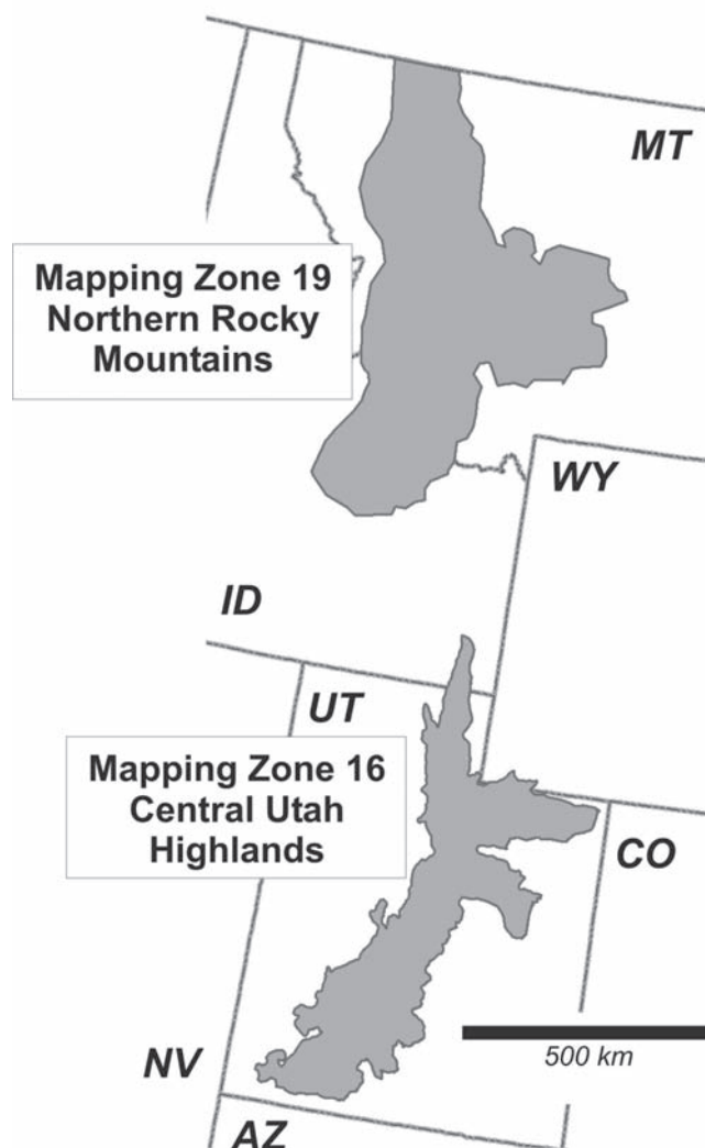
Figure 1 —The study areas for the LANDFIRE Prototype Project were located in the central Utah highlands (Mapping Zone 16) and the Northern Rocky Mountains (Mapping Zone 19). LANDFIRE used mapping zones delineated for the Multiple Resolution Land Cover (MRLC) 2001 Project ( http://landcover.usgs.gov/index.asp ). All of the 24 core LANDFIRE Prototype products were produced for each zone. Lessons learned in the central Utah study area resulted in refinements that were applied in the northern Rocky Mountains.
