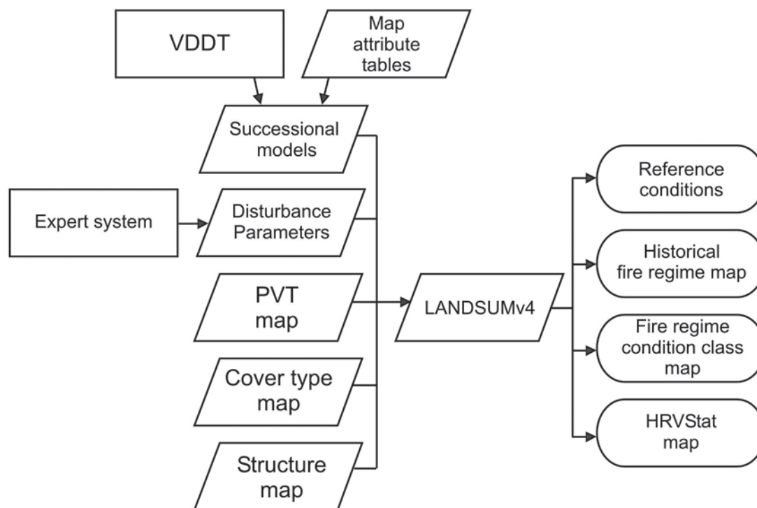
Figure 6 —The LANDFIRE fire regime and ecological departure mapping procedure. Successional models were developed for each mapped PVT. These models, along with the PVT map and a suite of disturbance and weather parameters developed from empirical modeling or acquired from expert opinion, were implemented within the LANDSUMv4 landscape fire succession model to simulate spatial time series of vegetation characteristics and wildland fire. This information was summarized using the Interagency Fire Regime Condition Class Guidebook methods and the HRVStat software application to create maps of simulated historical fire regimes and departure from historical vegetation conditions.
