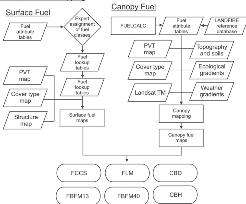
Figure 7 —The LANDFIRE fuel mapping procedure. Surface fuel was mapped using a rule-based approach in which combinations of LANDFIRE map classes were matched with both fire behavior fuel models and fire effects models. These look-up tables and the LANDFIRE vegetation maps were used to create the final LANDFIRE surface fuel maps. Canopy fuel (crown base height and crown bulk density) was mapped with a predictive landscape modeling approach using Landsat imagery and a suite of biophysical gradient layers.
