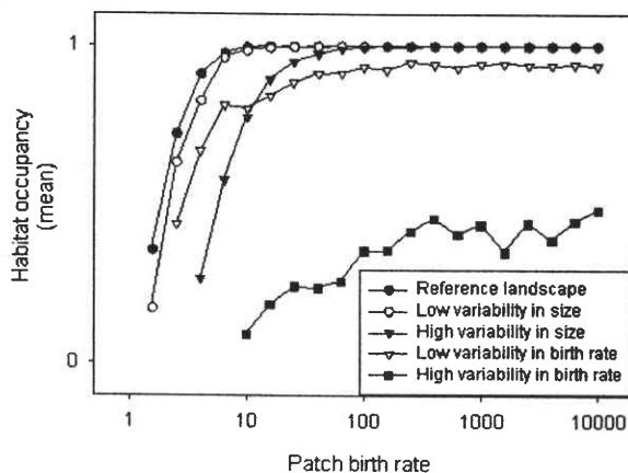
Fig. 6. A profile of habitat occupancy in a typical patchy population ( \lambda = 1.1 , patch size A = 10 ). Shown is a disturbance model with short patch lifetimes (3.1 yr). Habitat occupancy is the mean proportion of habitat occupied by the species over time.
