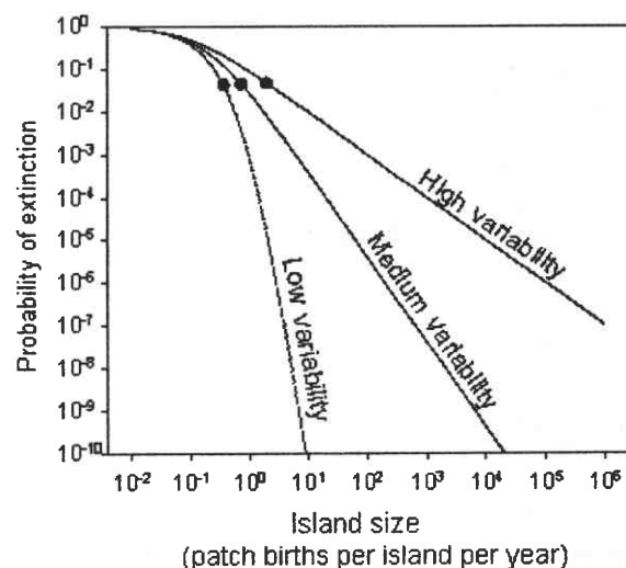
Fig. 9. The concept of landscape stochasticity in the context of island biogeography theory. The island-wide "gap" effect for a species shows an approximate power relationship with island size. The slope of the relationship is related to variability in the patch birth rate. The three dots mark the location of critical thresholds on each curve, indicating the points at which it becomes highly unlikely that the species can persist on the island for even a short time.
