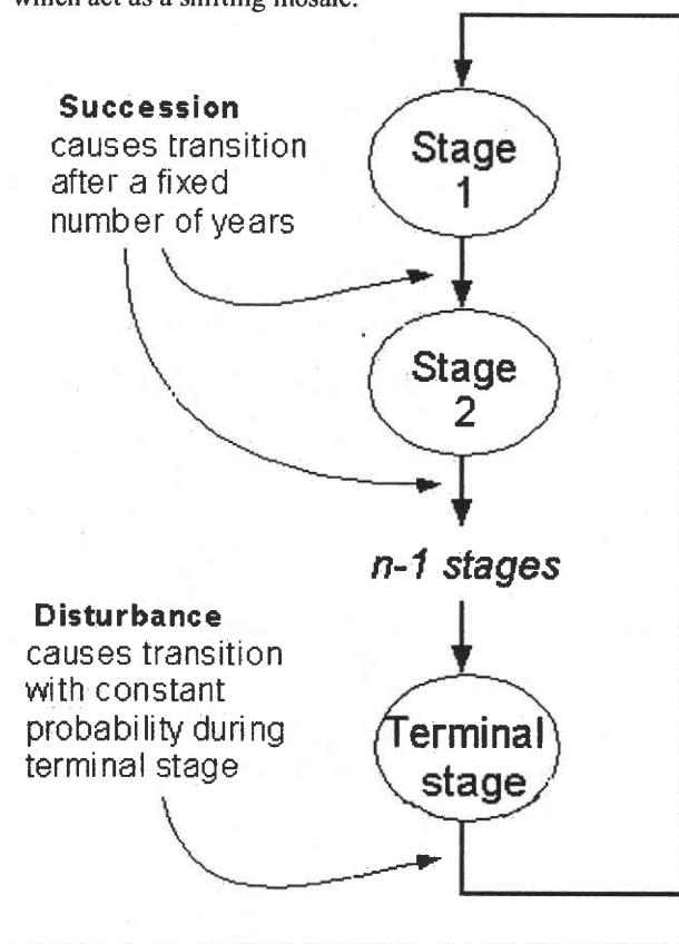
Fig. 1. A diagram of the succession concept assumed by the model. Successional patches transform into the next stage after a certain number of years. At the terminal stage, the patch is destroyed by disturbance, resetting it to the initial stage. A landscape consists of a population of such patches, which act as a shifting mosaic.
