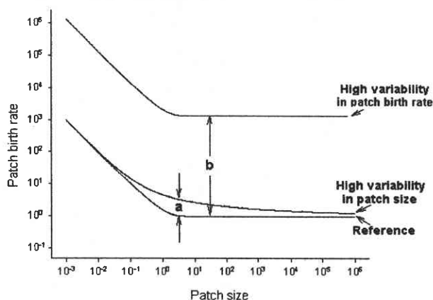
Fig. 4. The effect of landscape stochasticity on the position of the threshold. The reference curve is the critical threshold shown in Fig. 2 (successional patches with lifetime = 3.1 yr). The middle curve is the critical threshold for similar landscapes differing only in that they have high variability in patch sizes ( u_A = 10 ). The upper curve is the critical threshold for landscapes that have high variability in patch births per year ( u_B = 10 ). The lengths of arrows a and b are examples of gap effects for particular scenarios.
