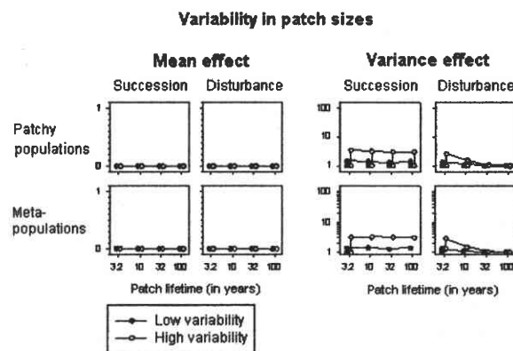
Fig. 7. The mean and variance effects when patch sizes were variable: u_A = 1 (low), and u_A = 10 (high). Larger effects imply higher risks of species extinction. The horizontal curves illustrate effects for species with medium demographic rates ( \lambda = 1.25 for patchy populations, and c = 0.001 for metapopulations). The vertical lines illustrate the range of effects observed under high and low demographic rates ( \lambda = 1.01 – 2.0 , and c = 0.1 – 0.00001 ). For the mean effect, effect size was always close to zero, and there was virtually no spread among the different demographic rates. For the variance effect, effect size was only negligible in species with low demographic rates ( \lambda = 1.01 , c = 0.00001 ; not labeled in figure), or in patches with long lifetimes and disturbance as the mechanism of turnover.
