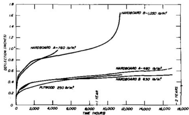
Figure 5. — Plot of deflection versus time for 6-foot I-beams in cyclic humidity environment. (M 145 681)
