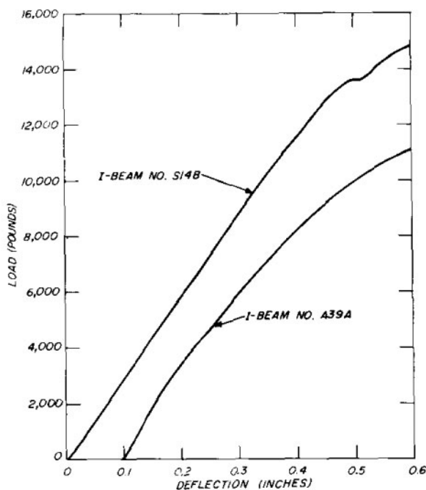
Figure 6. — Load-deflection curves for 6-foot hardboard-webbed I-beams tested after 17,000 hour exposure to cyclic humidity environment. (M 145 683)
