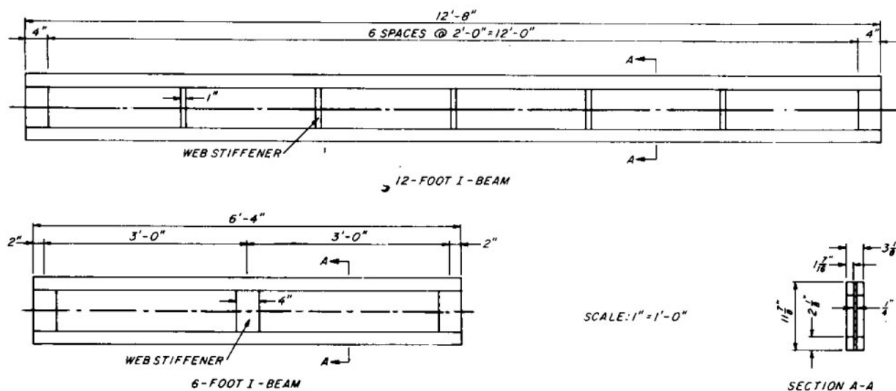
Figure 1. — Details of the 6-foot and 12-foot I-beams used in this study. (M 143 780)
