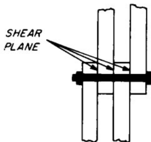
FOUR-MEMBER JOINT
