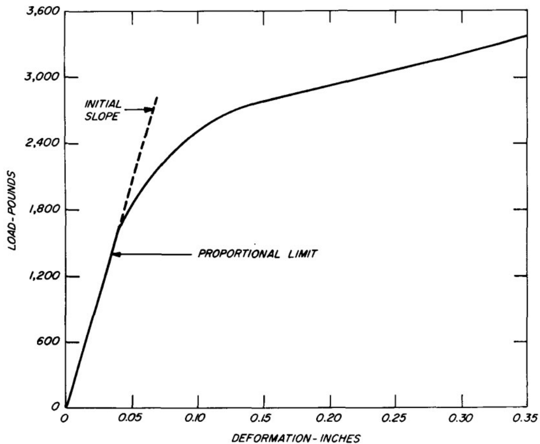
Figure 5.—Typical load-deformation curve for center member, and 3-in. side members). three-member bolted Joint (3/8-in. bolt, 2-in. (M144964)
