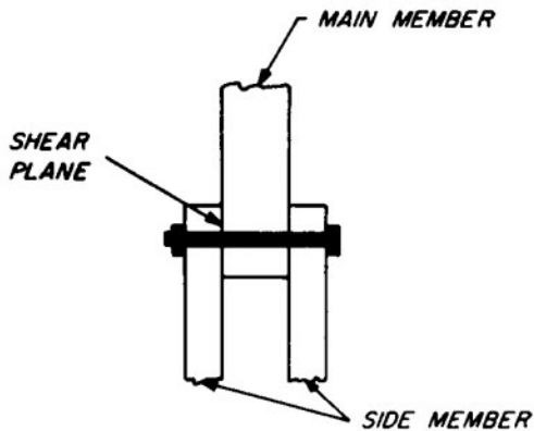
THREE-MEMBER JOINT
