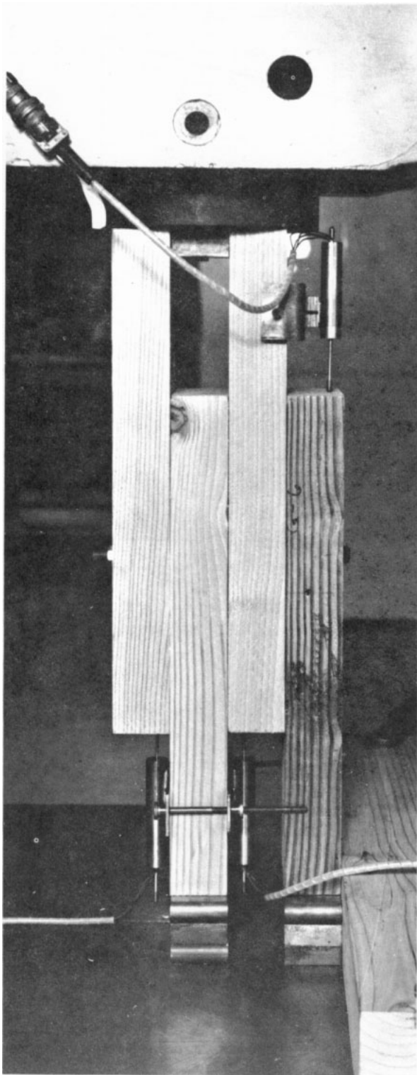
Figure 4.—Testing of four-member joints showing position of transducers. (M 144 227)
