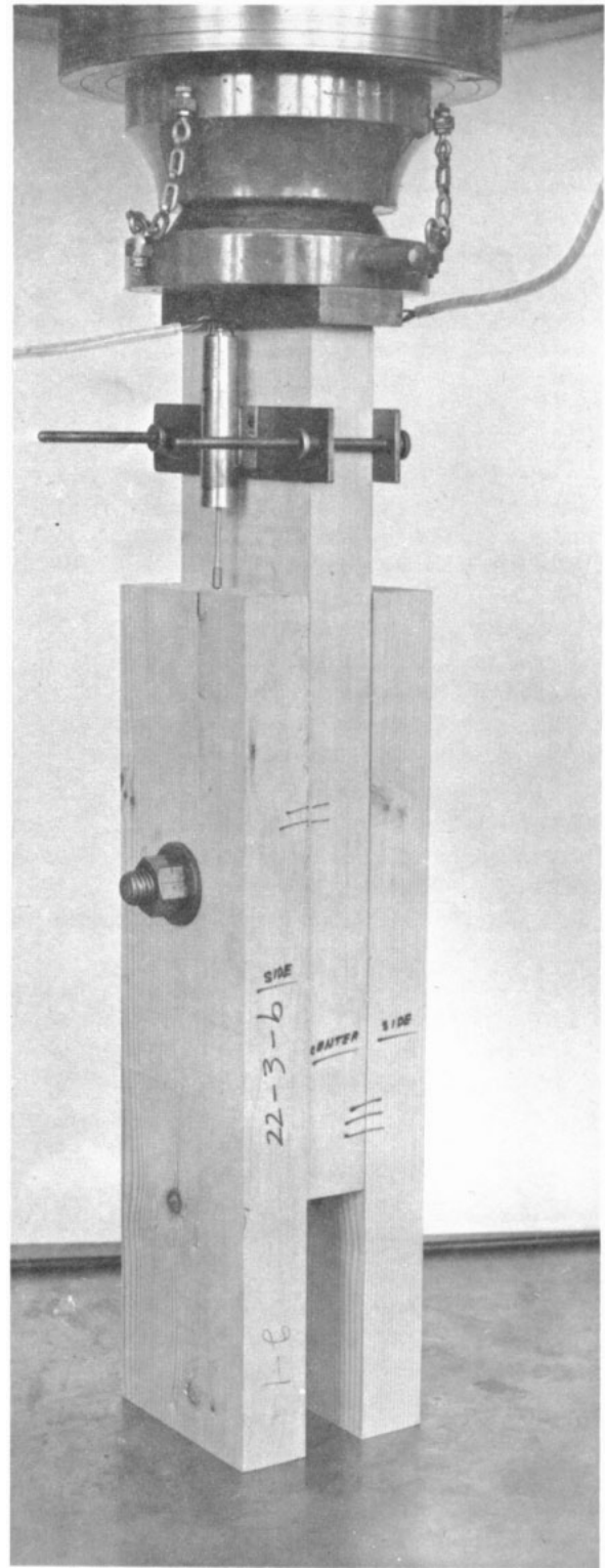
Figure 3.—Testing arrangement with three- member joints. (M 143 715)
