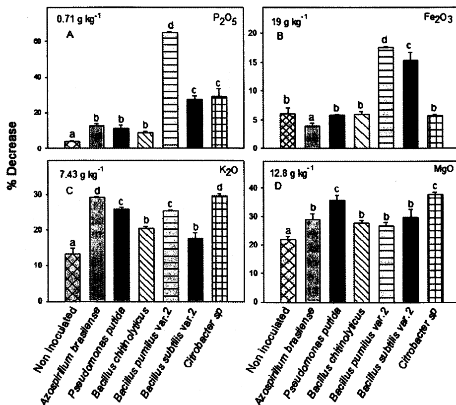
Fig. 5 Removal of P 2 O 5 , K 2 O, Fe 2 O 3 , and MgO from the rock substrate in which cardon cacti inoculated with rhizoplane bacteria were grown for 12 months. Numbers in each sub-figure represent the initial concentration of each element in crushed rock. Results are presented as percentage decrease of the mineral. Columns denoted by a different letter in each sub-figure differ significantly at p \leq 0.05 by one-way ANOVA. Bars represent standard error (SE).
