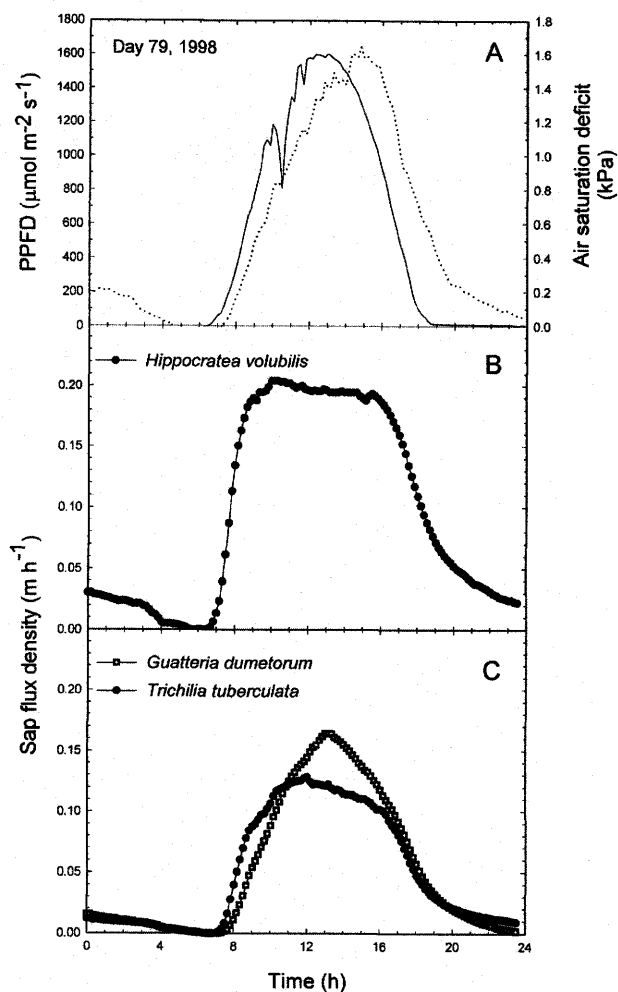
Fig. 5 Diurnal courses of a photosynthetic photon flux density (PPFD, solid line) and air saturation deficit (ASD, dotted line), b basal sap flux density for the liana Hippocratea volubilis , and c basal sap flow for the tree species Guatteria dumetorum and Trichilia tuberculata , on 20 March 1998 (day 79)
