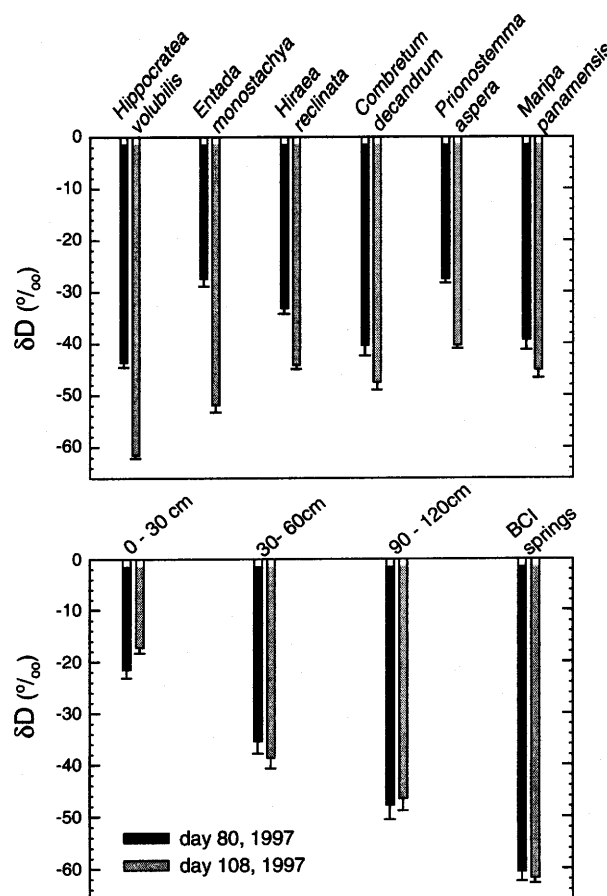
Fig. 2 Average xylem sap delta deuterium ( \delta D ) sampled on 21 March (day 80) and 18 April (day 108), 1997 for six liana species ( n=4 plants; upper panel) and soil and springs \delta D sampled on the same dates ( n=6 samples; lower panel) on Barro Colorado Island, Panama
