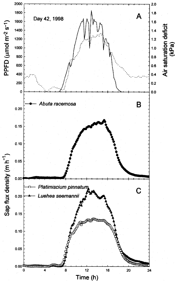
Fig. 3 Diurnal courses of a photosynthetic photon flux density (PPFD, solid line) and air saturation deficit (dotted line), b basal sap flux density for the liana Abuta racemosa , and c basal sap flow for the tree species Luehea seemannii and Platimiscium pinnatum , on 11 February 1998 (day 42)
