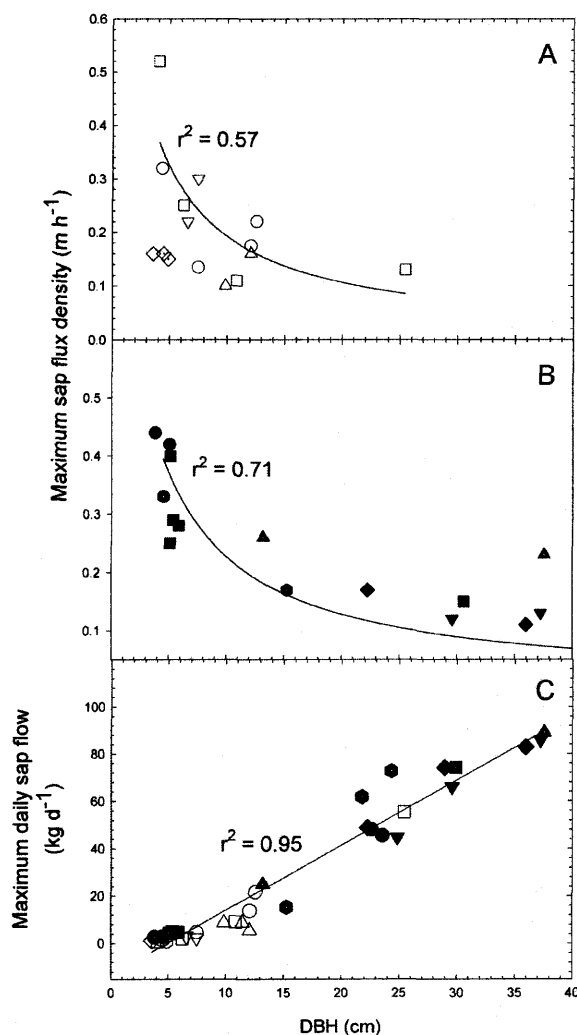
Fig. 6 a , b Maximum sap flux density and c maximum daily sap flow for lianas (open symbols) and branches and trees (closed symbols) as a function to diameter at breast height. Open circle Hippocratea volubilis , open square Entada monostachya , open diamond Clitoria javitensis , open triangle Abuta racemosa , diamond with a dot within Combretum decandrum , open inverted triangle Prionostemma aspera , black circle Trichilia tuberculata , black square Luehea seemanii , black triangle Platimiscium pinnatum , black inverted triangle Quararibea asterolepis , black diamond Alseis blackiana , dark bordered circle Ficus insipida , dark bordered square Guatteria dumetorum , hexagon Ochroma pyramidale , circle with a dot within Cecropia obtusifolia . Values for tree branches from 4 to 6 cm diameter were measured in 1997 and other values were measured in 1998
