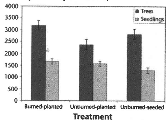
FIGURE 3. Mean tree and seedling density across treatments. Error bars represent one standard error of the mean.
