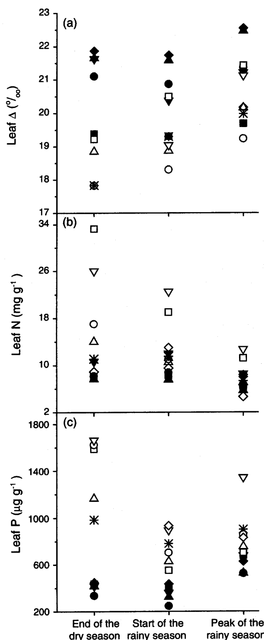
Fig. 5 Seasonal changes in leaf a C isotopic discrimination \Delta , b N and c P concentrations for evergreen and deciduous species growing in a cerrado site at the Instituto Brasileiro de Geografia e Estatística reserve. Leaf samples were collected on 17 September or 6 October 1995 (end of dry season), 2 November 1995 (start of rainy season) and 7 March 1996 (peak of rainy season). Evergreen species: ■ S. macrocarpa , ● M. ferruginata , ▲ R. montana , ▼ S. paniculatum , filled diamond V. elliptica , asterisk O. hexasperma . Deciduous species: □ D. miscolobium , ○ P. pubescens , △ Q. grandiflora , ▽ K. coriacea ◇ Q. parviflora . There were statistically significant differences ( P < 0.05 ; Fisher's PSLD test) between evergreen and deciduous species in terms of leaf \Delta , N and P. At the community level, leaf N concentrations were significantly different between the end of the dry period and the peak of the rainy period and between the start and the peak of the rainy period. In terms of leaf P concentrations, there were significant differences between the end of the dry and the start of the rainy season and between the start and the peak of the rainy season. There was no significant effect of seasonality on leaf \Delta
