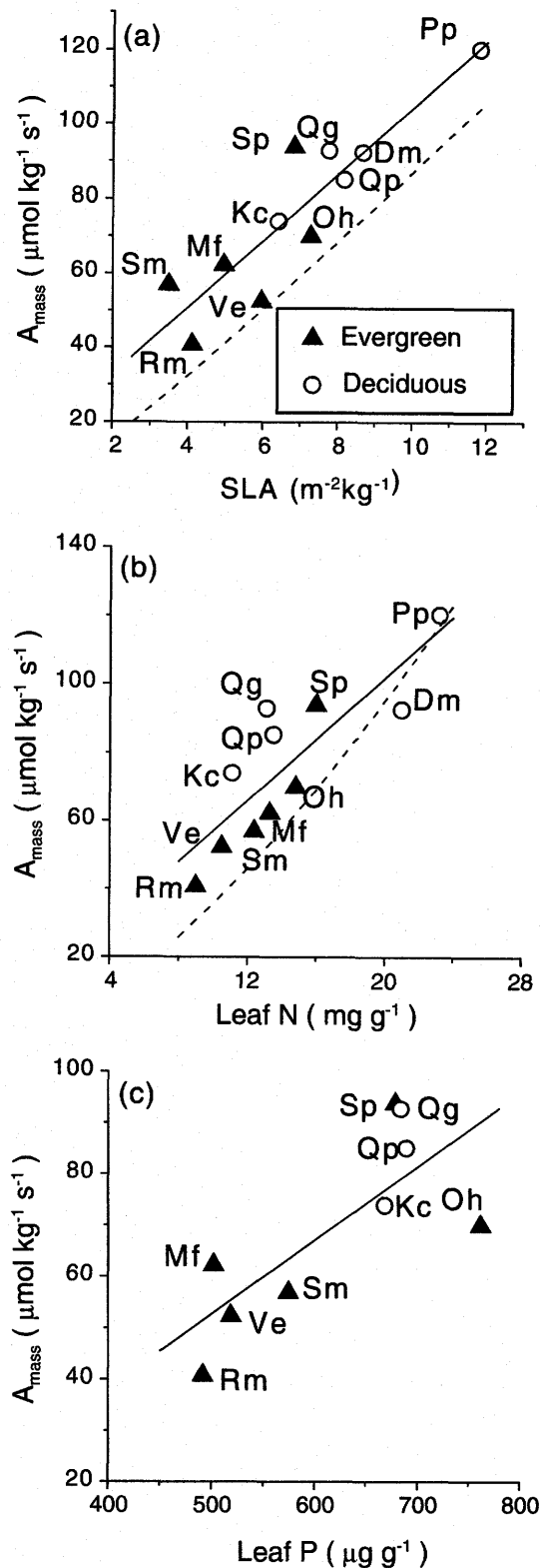
◀ Fig. 1 Relationships between a maximum \text{CO}_2 assimilation on a mass basis ( A_{\text{mass}} ) and specific leaf area (SLA); b A_{\text{mass}} and leaf N concentration; c A_{\text{mass}} and leaf P concentration. Each point is the mean of two to six trees per species. The lines are regressions fitted to the data: a A_{\text{mass}} = 15.108 + 8.9262(\text{SLA}) , r = 0.901 , P < 0.001 , n = 11 ; b A_{\text{mass}} = 12.132 + 4.4782(\text{leaf N}) , r = 0.841 , P = 0.001 , n = 11 ; c A_{\text{mass}} = -19.221 + 0.1438(\text{leaf P}) , r = 0.766 , P = 0.016 , n = 9 . The dotted line describes the log-log relationship between A_{\text{mass}} and SLA ( \log A_{\text{mass}} = -0.22 + 1.08 \log_{10} \text{SLA} ; Reich et al. 1999) and between A_{\text{mass}} and leaf N [ \log A_{\text{mass}} = 0.13 + 1.42 \log_{10}(\text{leaf N}) ; Reich et al. 1999] fitted to data from six biomes. Sm Schefflera macrocarpa , Mf Miconia ferruginata , Rm Roupala montana , Sp Sclerolobium paniculatum , Ve Vochysia elliptica , Oh Ouratea hexasperma , Dm Dalbergia miscolobium , Pp Pterodon pubescens , Qp Qualea parviflora , Qg Q. grandiflora , Kc Kielmeyera coriacea .
