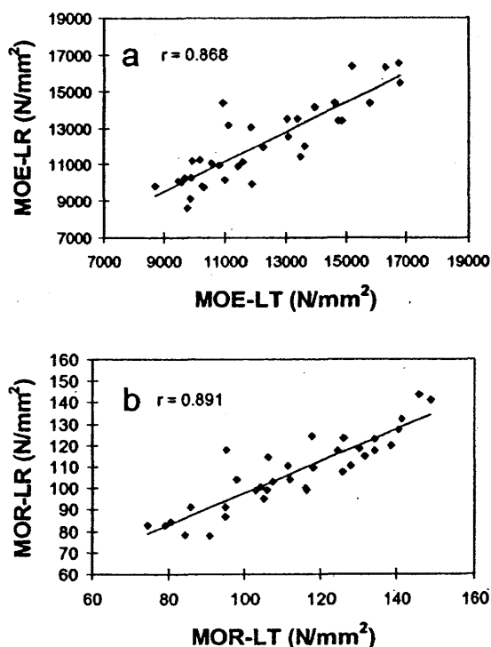
FIG. 3. Correlation of MOE-LT to MOE-LR and MOR-LT to MOR-LR; each point represents a tree, and the x- and y-values are the means of four samples each.
