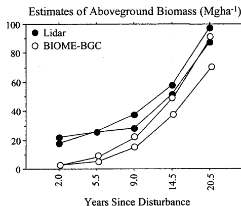
Fig. 7. Estimates of aboveground biomass (Mg ha -1 ) as a function of years since disturbance, for two methods: lidar predictions and Biome-BGC model results. Results from each method have been split into two classes: above and below the 50th percentile aboveground biomass value for each dataset.
