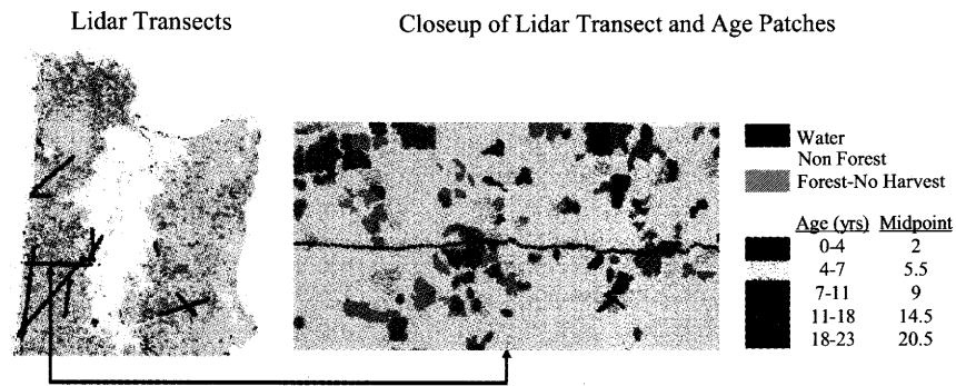
Fig. 2. Lidar transects and a sample of the mapped stand ages that are based on change detection analysis.
