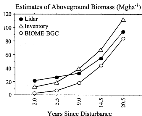
Fig. 6. Estimates of aboveground biomass (Mg ha -1 ) as a function of years since disturbance, from three methods: lidar predictions, Biome-BGC model results, and forest inventory plots.
