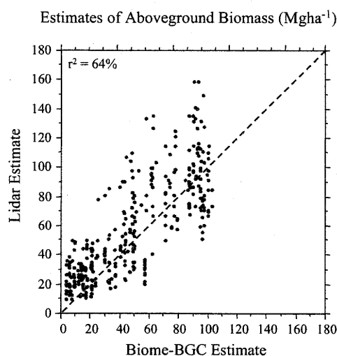
Fig. 5. Comparison of aboveground biomass (Mg ha -1 ) estimated from lidar/change detection and from Biome-BGC.
