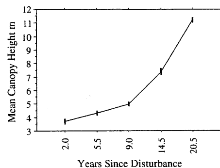
Fig. 4. Mean canopy height derived from lidar measurements as a function of years since disturbance. Error bars indicate one standard error.
