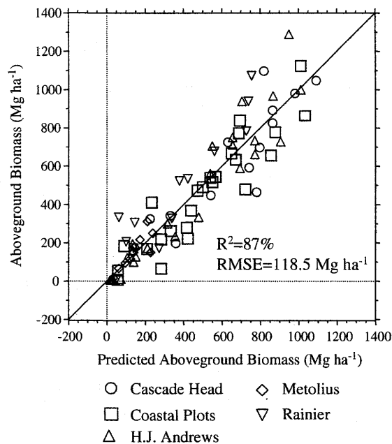
Fig. 3. Predicted and observed aboveground biomass for plots at the five sampling areas in western Oregon and Washington. This relationship explains 87% of variance, and none of the five areas showed significant differences in their slopes or intercepts from the overall equation.
