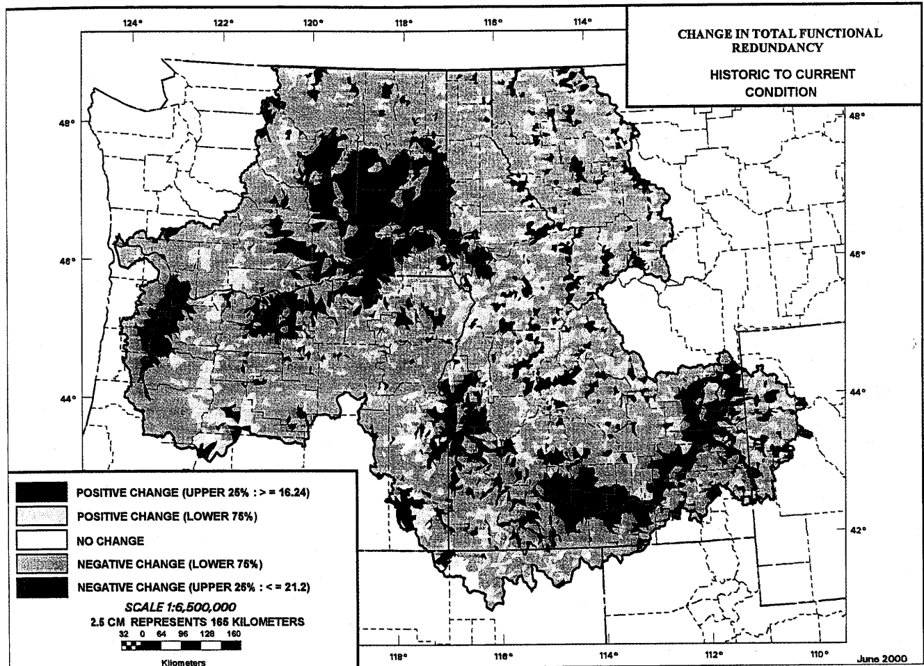
Fig. 1. Using GIS, Marcot et al. (2002b) depicted the concept of Total Functional Redundancy for the Columbia River Basin.
