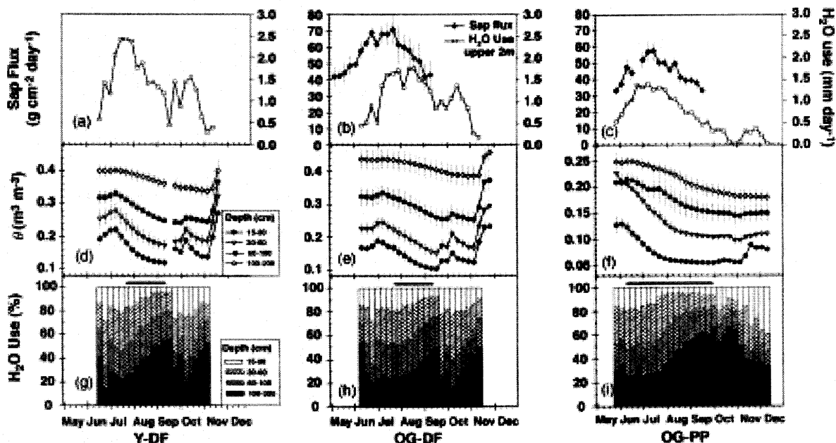
Fig. 2. Seasonal weekly water dynamics for young- and old-growth Douglas-fir stands (Y-DF, OG-DF), and for an old-growth ponderosa pine stand (OG-PP): (a–c) total daily water use from the upper 2 m soil profile based on fluxes in soil volumetric water content. Also depicted (b–c) total daily sap flux density \pm S.E. for trees in an old-growth Douglas-fir stand and an old-growth pine stand based on thermal dissipation probes installed 2 cm into sapwood at 2 m height. (d–f) Average seasonal decline in volumetric soil water content by depth \pm S.E. ( n = 4 ). (g–i) Relative water use from individual layers in the upper 2 m of the soil profile based on fluxes in soil volumetric water content. Horizontal bars at the top of (g–i) span the 2002 seasonal drought for each stand, and represent the period used for development of the soil water retention curves (Fig. 1).
