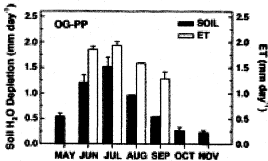
Fig. 8. Seasonal water loss from the old-growth ponderosa pine stand (OG-PP) based on volumetric soil water depletion in the upper 2 m of soil (soil H_2O depletion), or on eddy covariance measurements of site water vapor flux from a 47 m tower (evapotranspiration, ET). Soil water depletion was measured during 2002 and 2003. Eddy covariance measurements were made during 1996–1997 (Law et al., 2000a) and 2000 (Anthoni et al., 2002). Error bars represent the S.E. between years ( n = 2-3 ).
