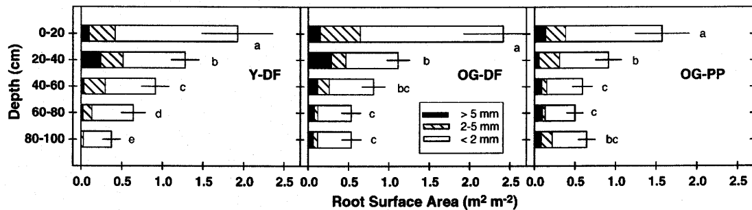
Fig. 6. Total root surface area for young- and old-growth Douglas-fir stands (Y-DF, OG-DF), and for an old-growth ponderosa pine stand (OG-PP) separated by size classes. Bars with the same letter within each site are not statistically different based on ANOVA and Duncan's multiple range test ( P < 0.05 ). Error bars represent \pm 1 S.E. about the mean total root surface area within each depth.
