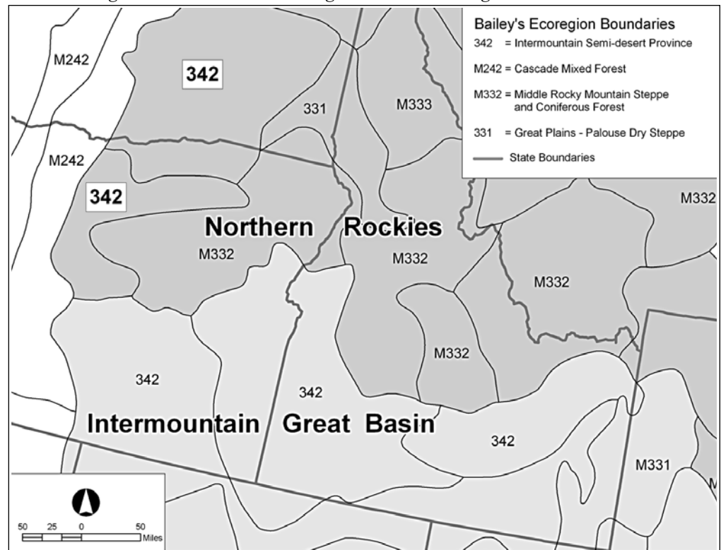
Figure 2.2. A polygon of an ecological province (342) that is embedded in the Northern Rockies bioregion is included in that bioregion to smooth bioregional boundaries.
