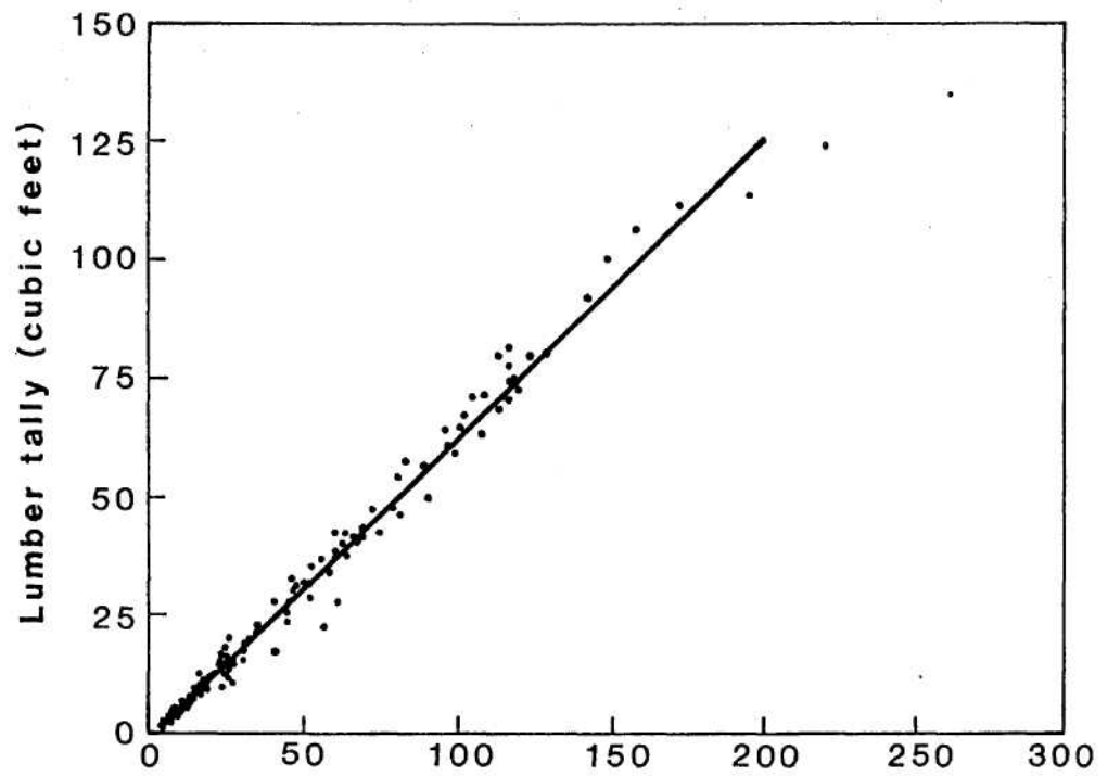
Figure 3—Regression line and data scatter of lumber tally (cubic feet) versus gross cubic log scale for sound incense-cedar logs. The regression equation is:
