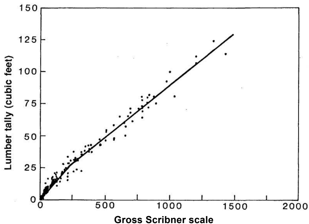
Figure 2—Regression line and data scatter of lumber tally (cubic feet) versus gross Scribner scale for sound incense-cedar logs. The regression equation is:
