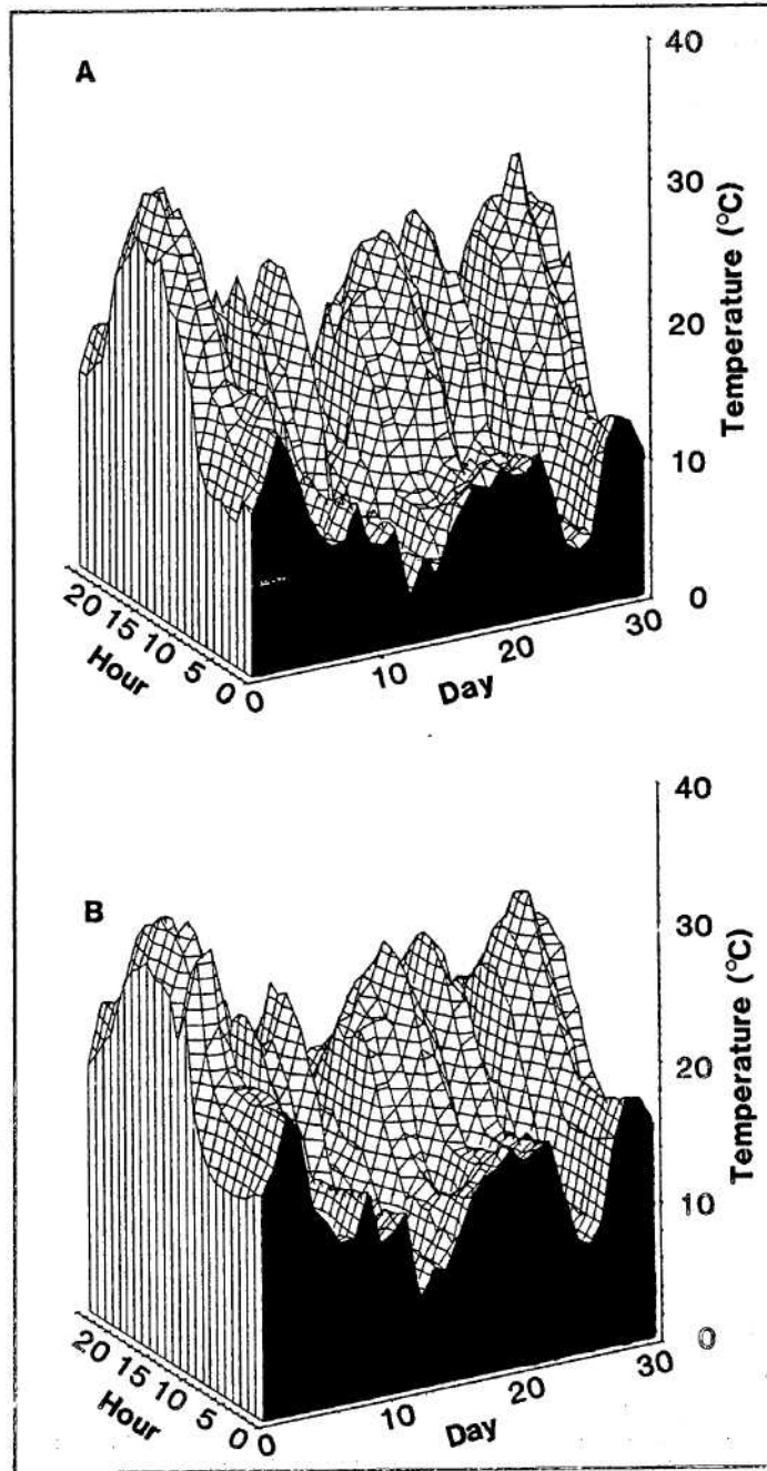
Figure 2—Air temperature at 1.3 m, July 27, 1985 (day 0), to August 28, 1985 (day 31): A, in clearcut; B, in uncut forest.
