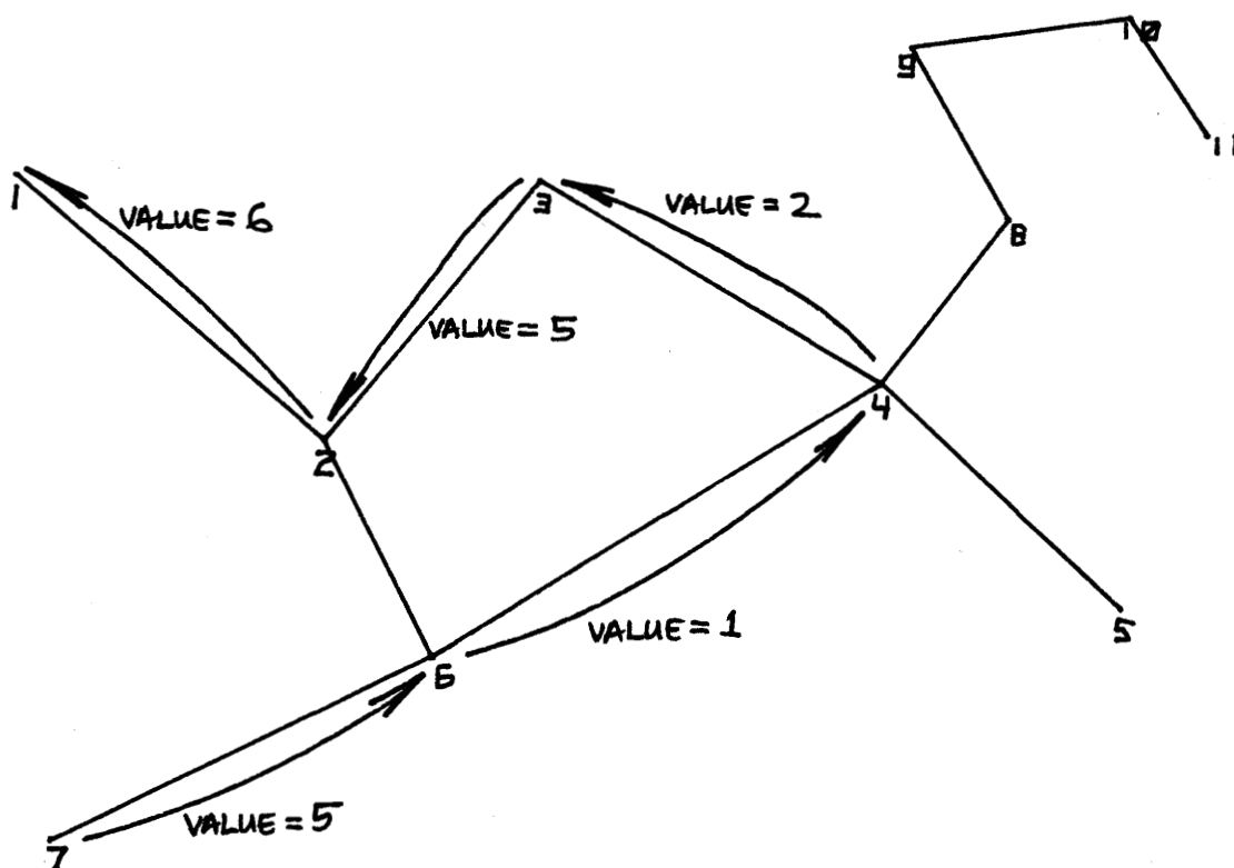
Figure 7.--The minimum path from node 7 to node 1, with link values for the selected links.
