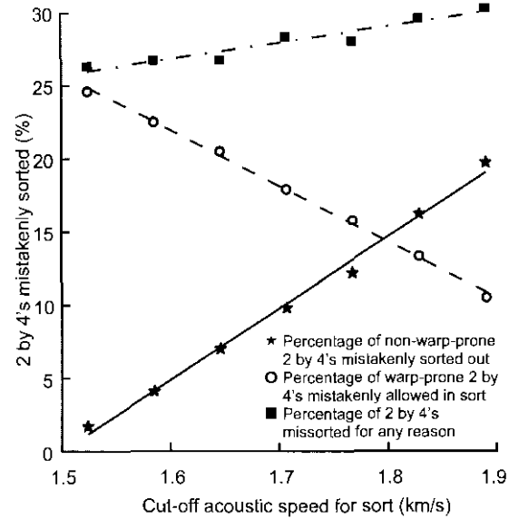
FIG. 4. Relationship between the percentage of ponderosa pine 2 by 4s mistakenly sorted and the cut-off acoustic speed.
