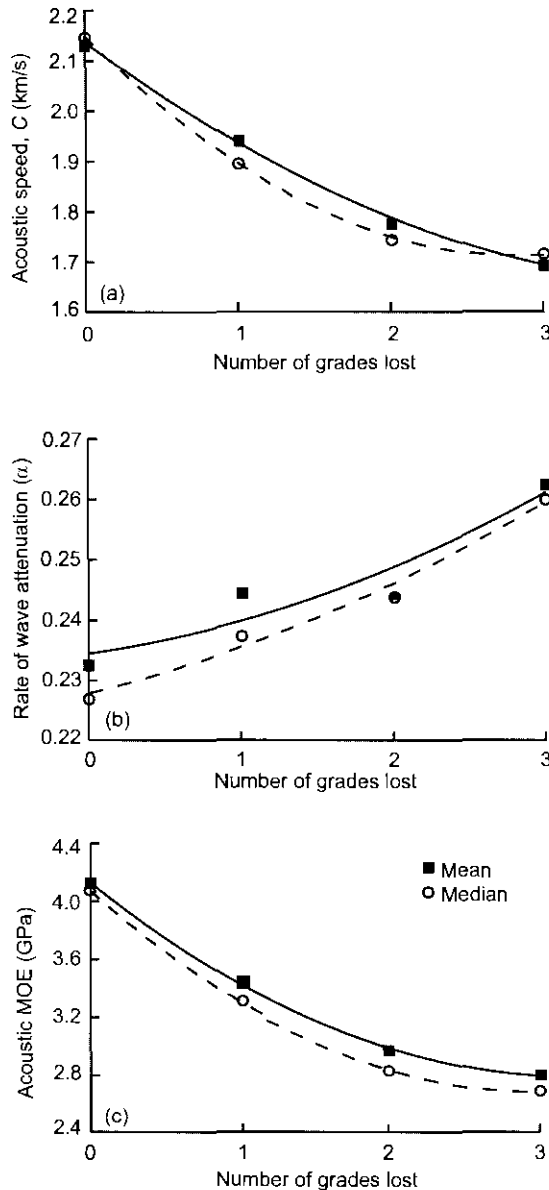
FIG. 3. Relationship between (a) acoustic speed length wise, (b) rate of wave attenuation, and (c) acoustic modulus of elasticity (MOE) of green ponderosa pine 2 by 4s and the number of grades lost from warp during kiln-drying.
