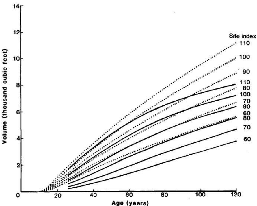
Figure 12. — A comparison of gross and net yield by age and site index at C.C.F. 175.
