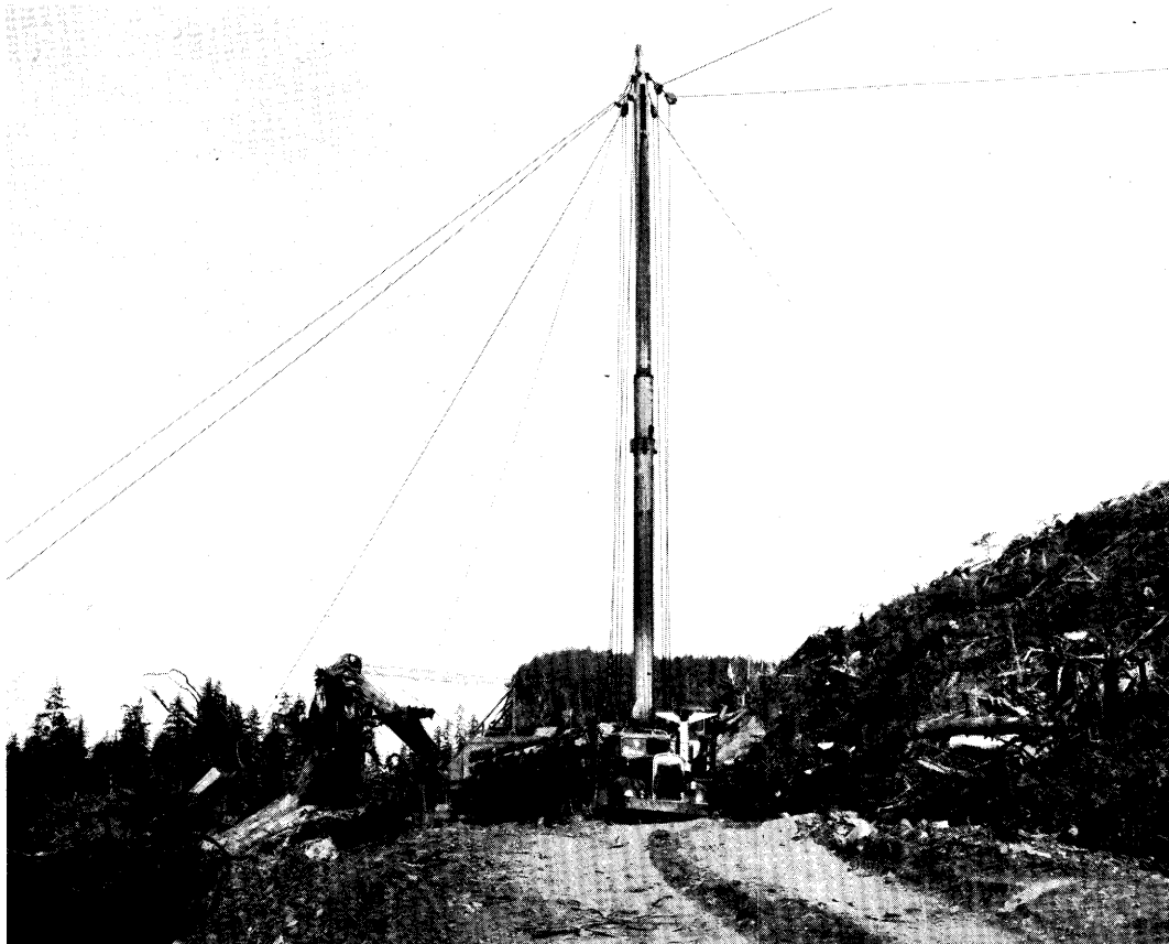
Figure 18.--A high-lead logging operation using a portable steel spar, Tongass National Forest, Alaska.
