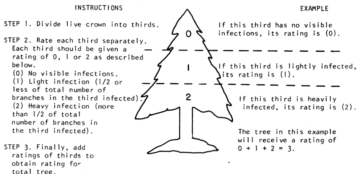
Figure 53.--The six-class mistletoe rating system (Hawksworth 1977).
