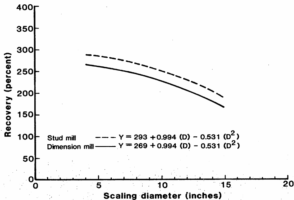
Figure 1.—Lumber recovery as a percent of net Scribner scale, by log scaling diameter.
