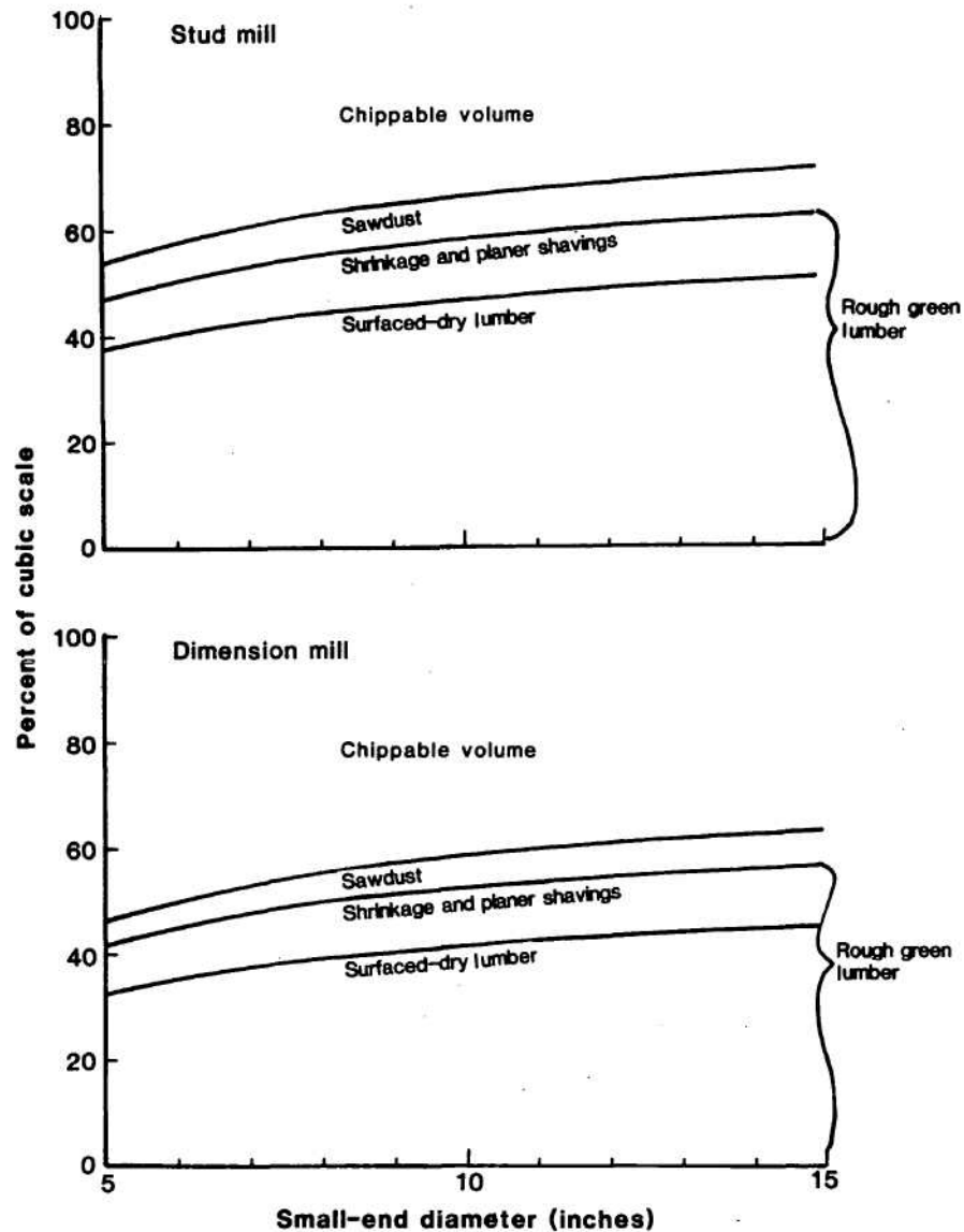
Figure 3.—Cumulative recovery and loss as a percent of cubic scale, by small-end diameter, for a stud mill and a dimension mill.
