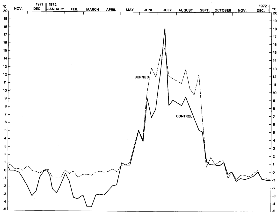
Figure 6.--Soil temperature at a depth of 5 cm in the organic layer at burned and unburned control sites during the 1st year after burning.
