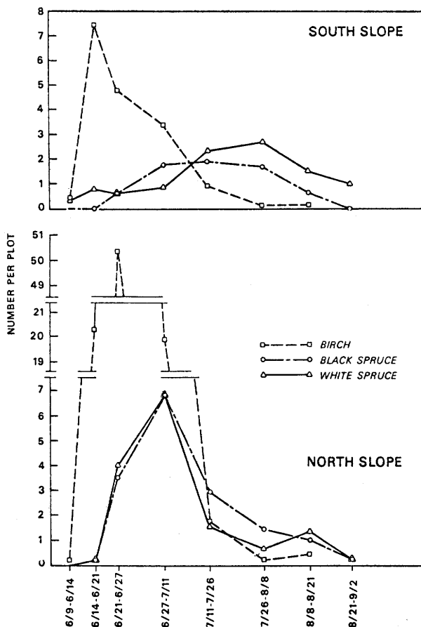
Figure 18.--Weekly germination of seeded birch, black spruce, and white spruce on north and south slopes 1 year after fire (1972).
