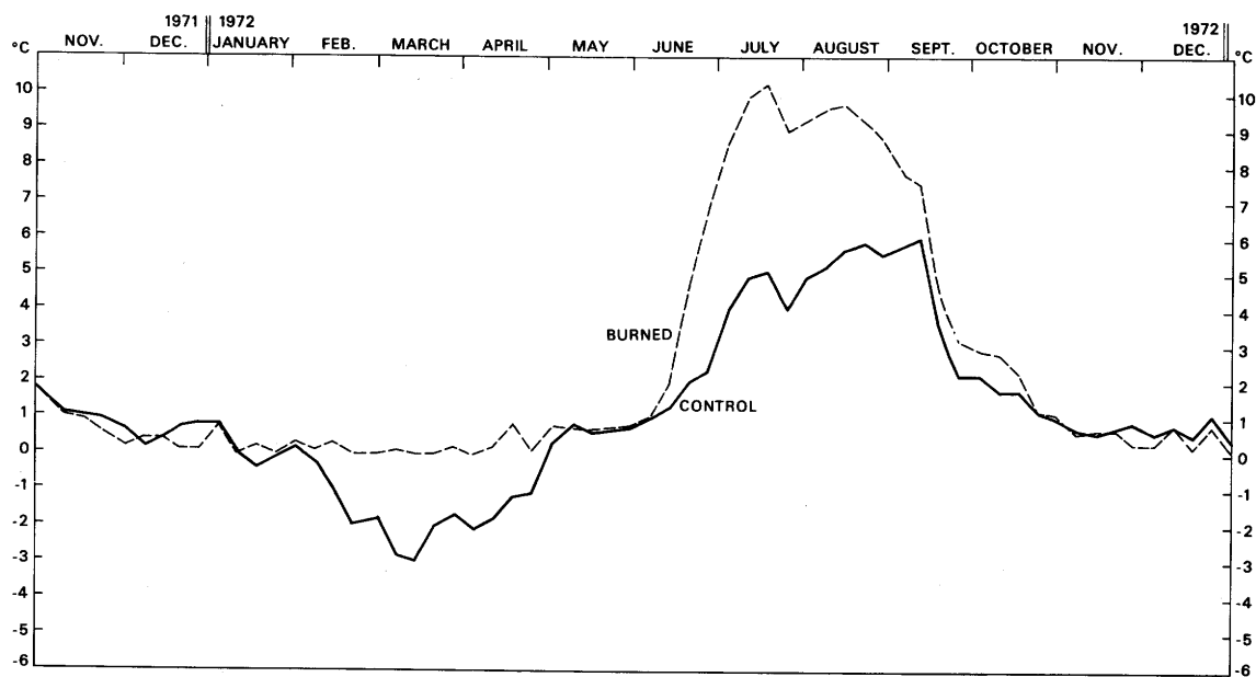
Figure 7.--Soil temperature at a depth of 10 cm in the mineral soil at burned and unburned control sites during the 1st year after burning.
