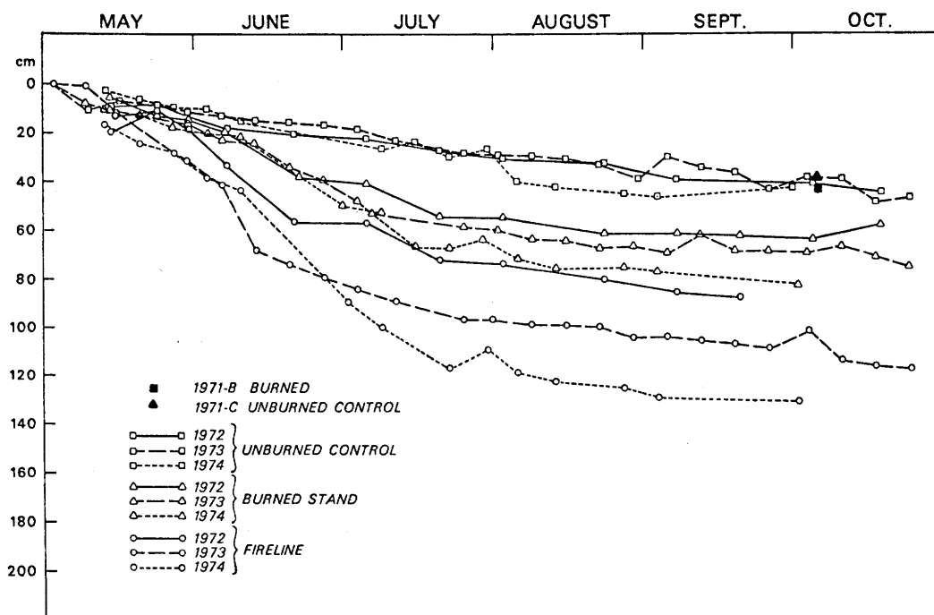
Figure 10.--Depth of thaw in a heavily burned stand, on a cleared fireline, and in an unburned control for 3 years after the fire.
