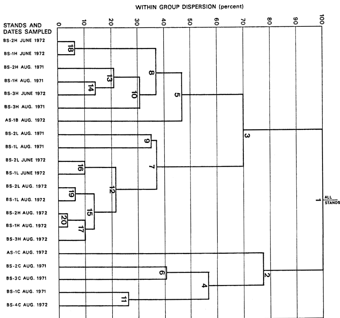
Figure 15.--Results of analysis of clusters of vegetation data (based on twenty 1-m 2 plots) collected in 11 sample stands over a 2-year period after the 1971 Wickersham Dome fire. For the within-group dispersion, a stand was treated as a new stand each time it was sampled. Burned stands were sampled in August 1971, June 1972, and August 1972; unburned controls were sampled only once.
