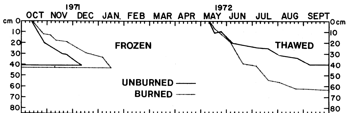
Figure 9.--Freeze-thaw cycle in a heavily burned stand and an unburned control for the 1st year after the fire. (Reproduced from: Viereck, Leslie A. 1973. Ecological effects of river flooding and forest fires on permafrost in the taiga of Alaska. In North American contribution, permafrost, second international conference, p. 66. Natl. Acad. Sci., Washington, D.C.).
