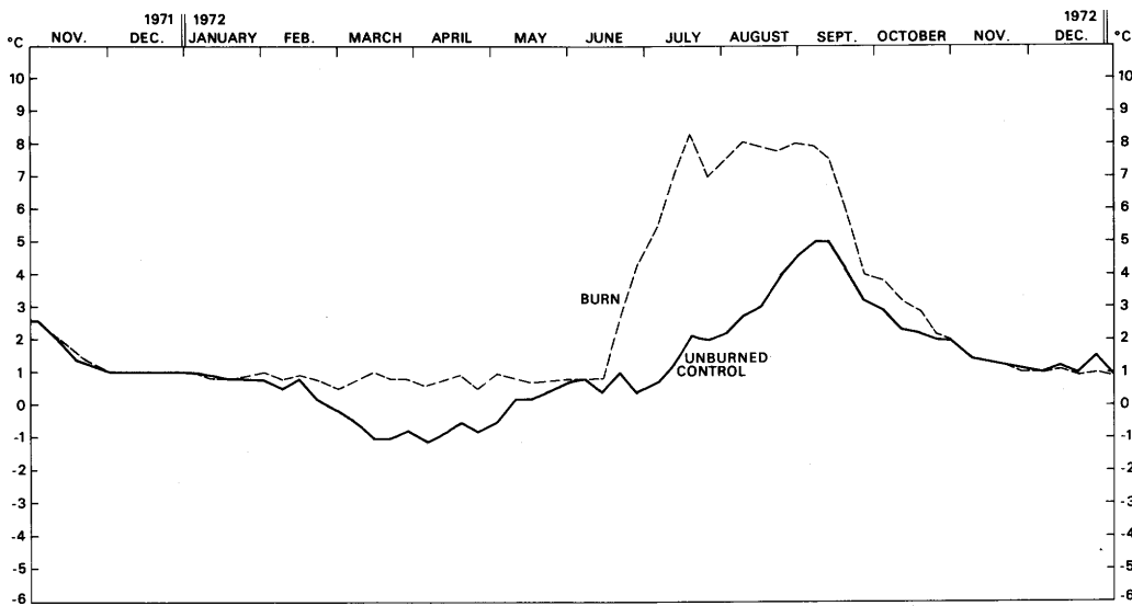
Figure 8.--Soil temperature at a depth of 50 cm in the mineral soil at burned and unburned control sites during the 1st year after burning.
