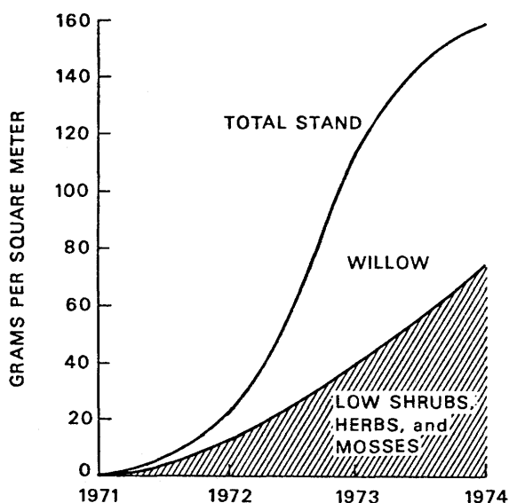
Figure 16.--Biomass of a heavily burned black spruce stand (BS-3H) for 4 years after the 1971 fire.
