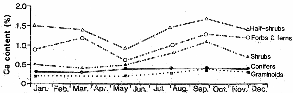
Figure 10.—Seasonal changes in the concentration of calcium.
