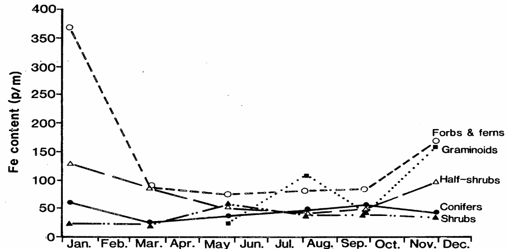
Figure 14.—Seasonal changes in the concentration of iron.
