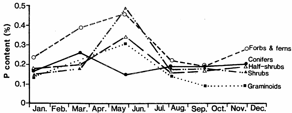
Figure 8.—Seasonal changes in the concentration of phosphorus.
