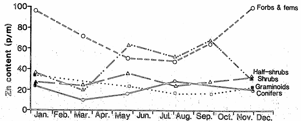
Figure 15.—Seasonal changes in the concentration of zinc.
