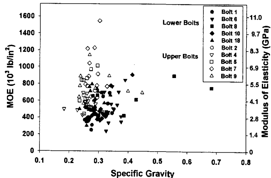
Fig. 12.12 Relationship of earlywood MOE to specific gravity.
