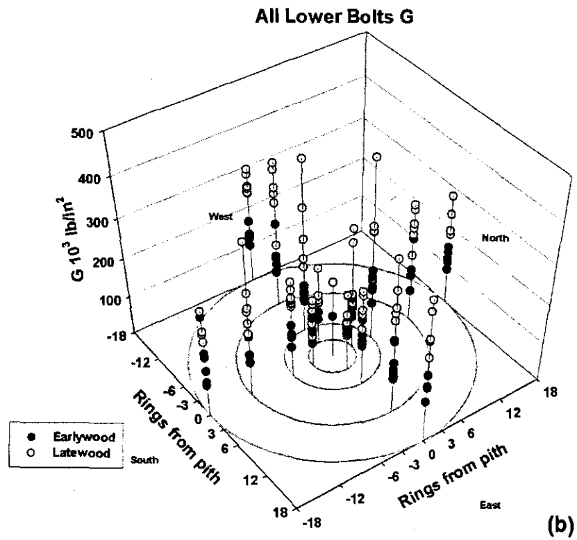
Fig. 12.21 Cardinal direction plots (a) for MOE and (b) for G of all lower bolts
