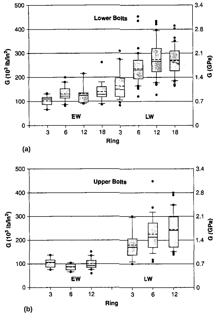
Fig. 12.6 Earlywood and latewood shear modulus (G) for lower and upper bolts.
