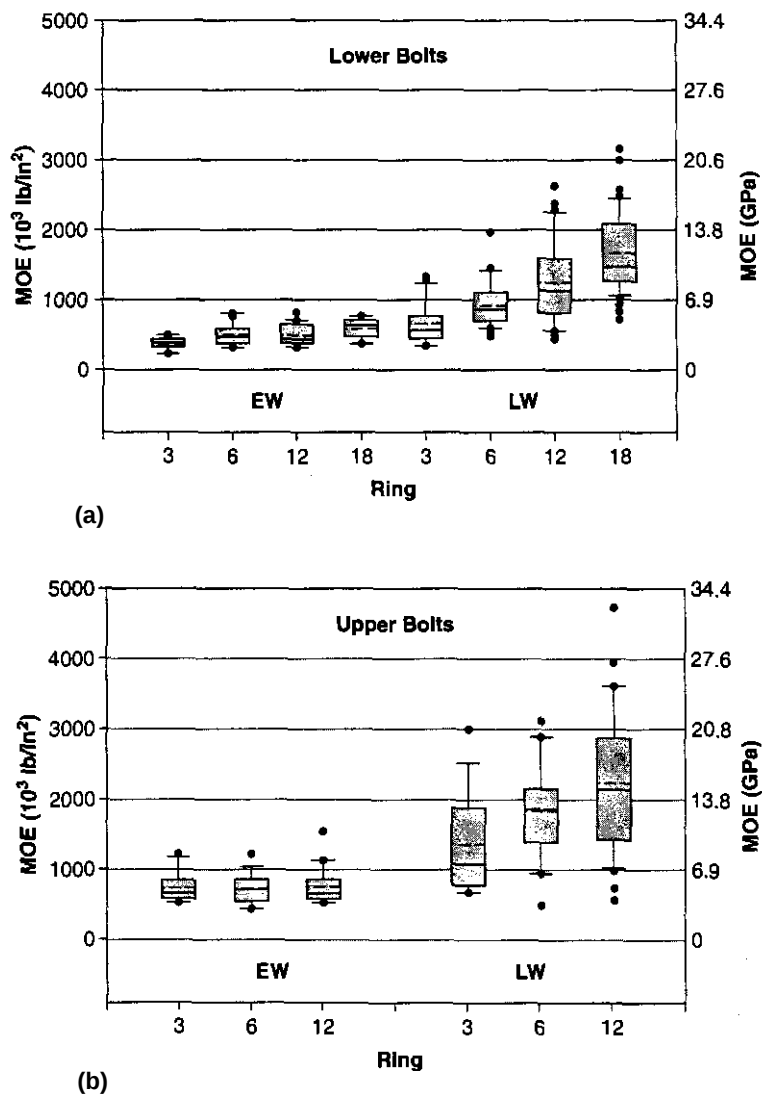
Fig. 12.5 Earlywood and latewood modulus of elasticity (MOE) for lower and upper bolts. Box plots show outlying data (dots); 5th, 25th, 50th, 75th, and 95th percentiles (solid lines); and mean values (dashed lines).
