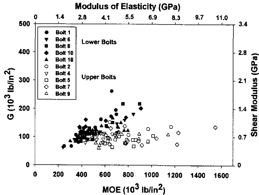
Fig. 12.11 Relationship of earlywood G to MOE.
