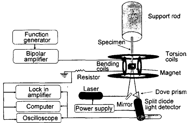
Fig. 12.3 Schematic of broadband viscoelastic spectrometry device. (This figure also is in the color section.)
