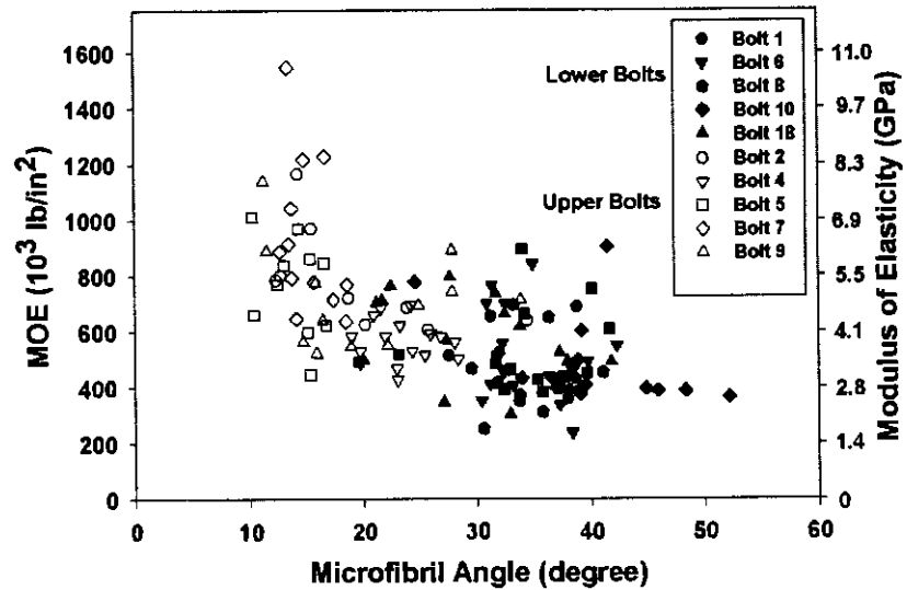
Fig. 12.13 Relationship of earlywood MOE to MFA.
