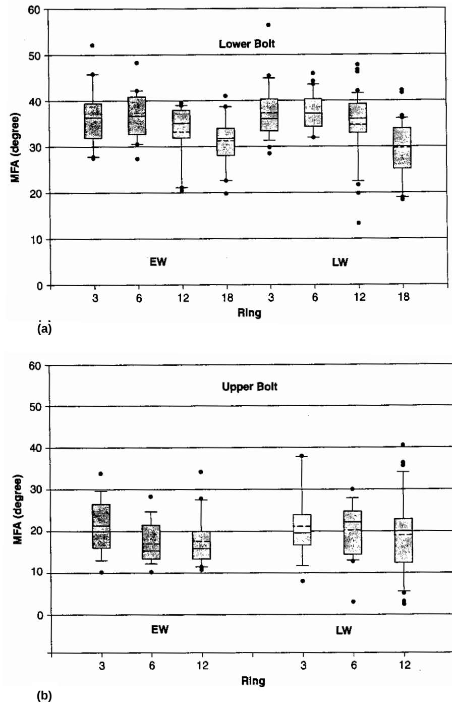
Fig. 12.8 Earlywood and latewood microfibril angles (MFA) for lower and upper bolts.
