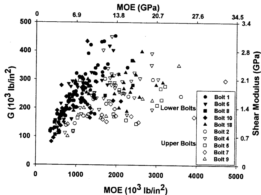
Fig. 12.15 Relationship of latewood G to MOE.
