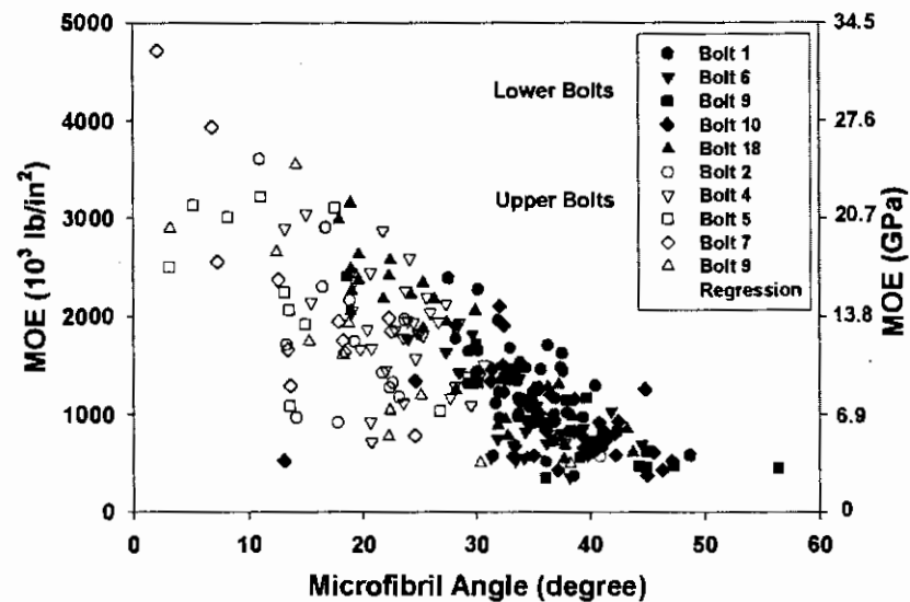
Fig. 12.18 Relationship of latewood MOE to MFA.
