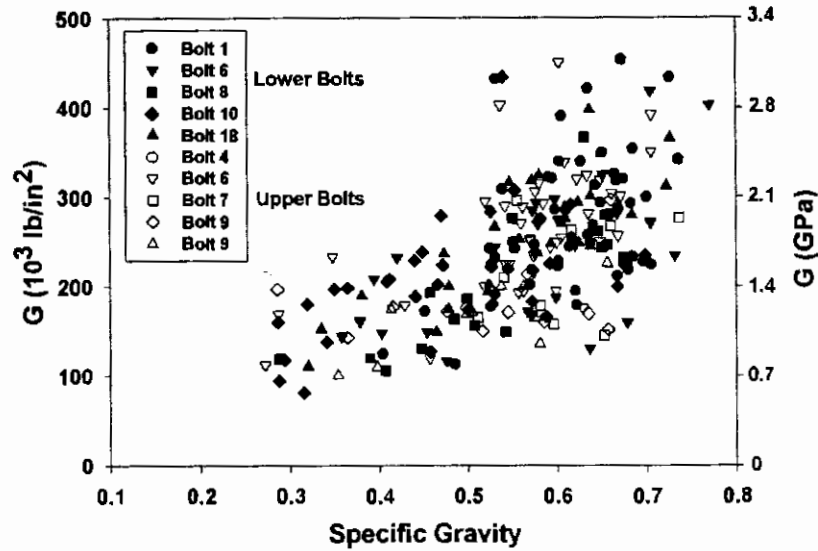
Fig. 12.17 Relationship of latewood G to specific gravity
