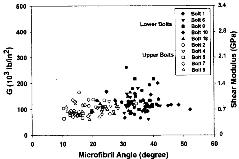
Fig. 12.14 Relationship of earlywood G to MFA.
