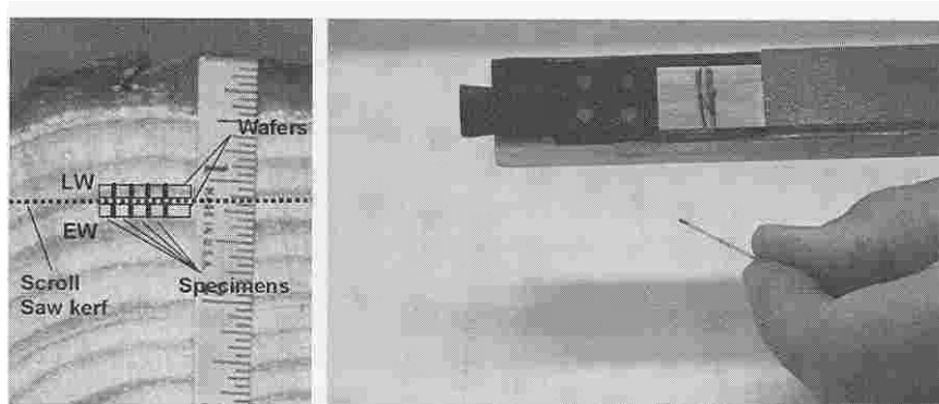
Fig. 12.2 Left , adjacent latewood (LW) and earlywood (EW) specimens were obtained for modulus of elasticity (E) and shrinkage evaluations. Right specimens were cut using a 1-mm-thick wafer held in place by a vacuum block. (This figure also is in the color section.)
