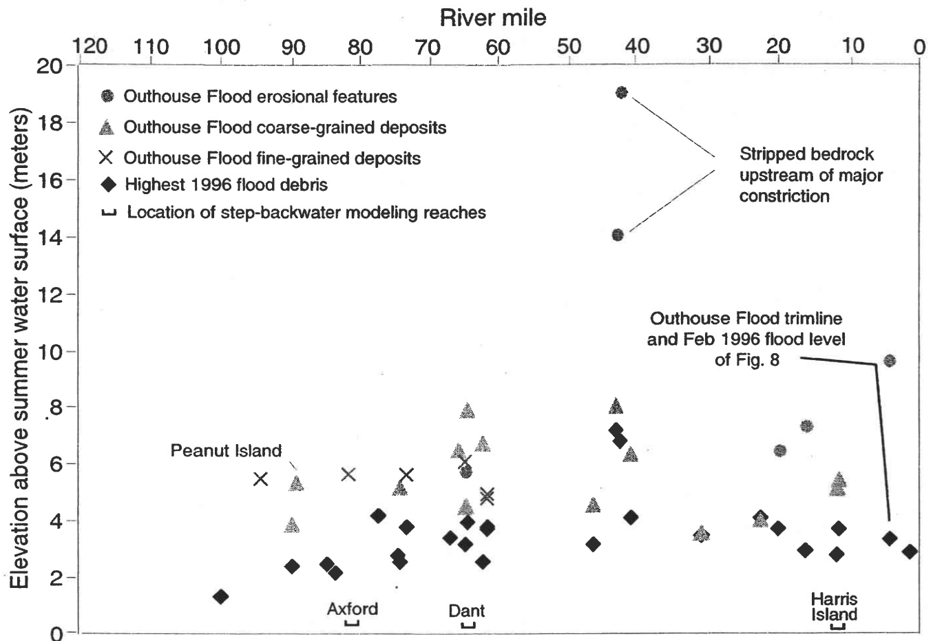
Figure 9. Comparison of the surveyed heights of paleostage evidence from the February 1996 flood and the Outhouse Flood.
