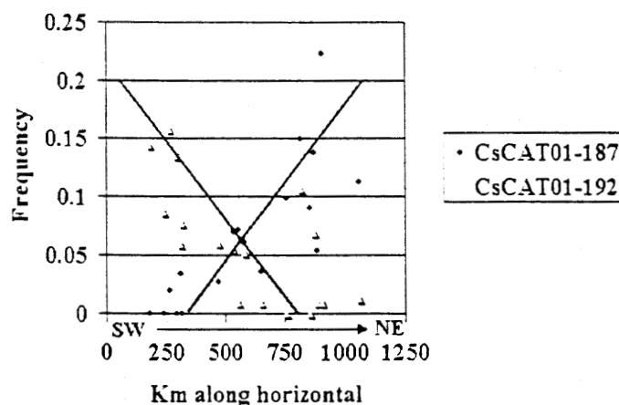
Figure 2. Plot of allele frequency by composite dependent variable (CDV) expressed in units of kilometers along horizontal.
