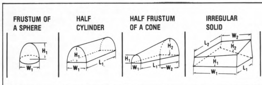
Figure 4.—Geometric solids and related dimensions used for estimating the volume of residue in piles.
