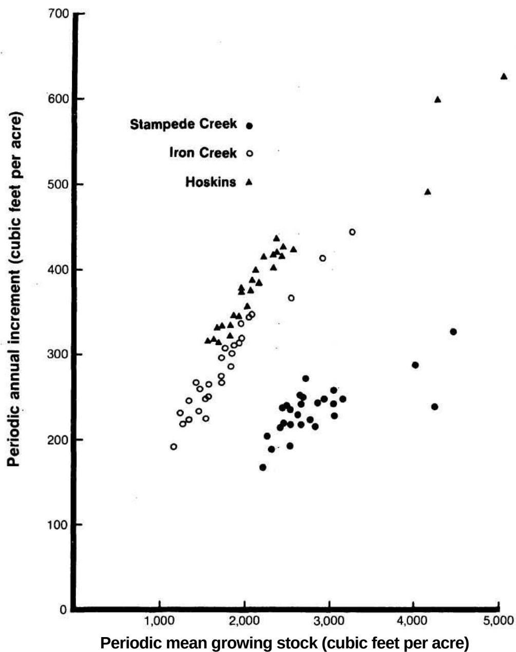
Figure 3.—Stampede Creek, Iron Creek, and Hoskins: periodic annual gross volume increment (trees 1.6 inches in d.b.h. and larger) in relation to volume of growing stock, first treatment period.
