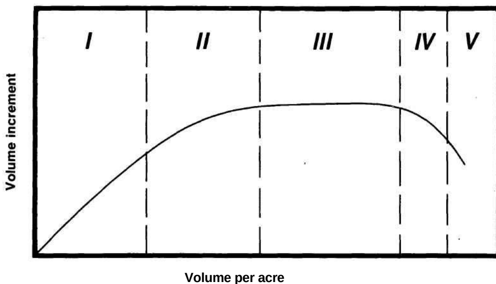
Figure 13.—Relation between standing volume and volume increment, as hypothesized by Langsaeter (prepared from Braathe 1957). Roman numerals denote Langsaeter's "density types."
