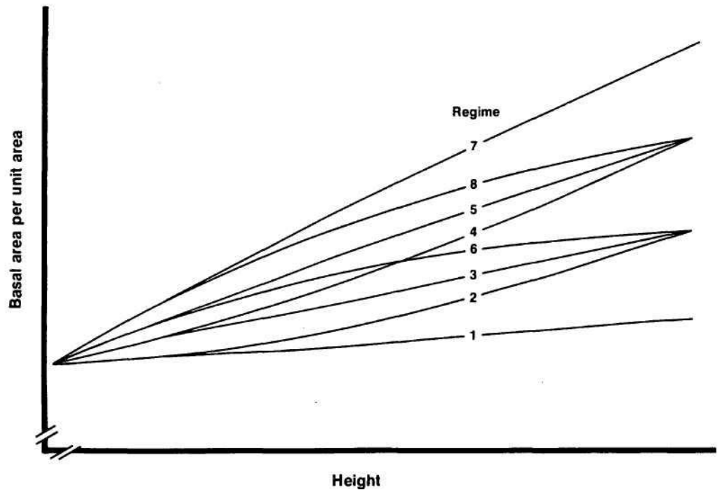
Figure 2.—Levels-of-growing-stock study in Douglas-fir: idealized trends of basal area for the eight thinning regimes.
