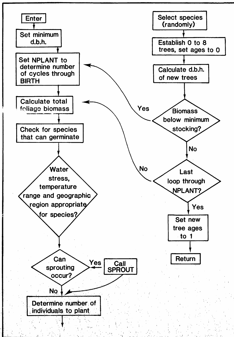
Figure 3 –Flow Chart for subroutine BIRTH.
