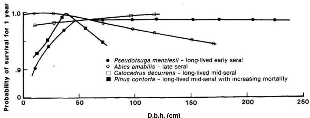
Figure 13.—Probability of tree survival 1 year after slow growth (less than 1 mm [0.04 in] of diameter increment) for four successional classes. A fifth class, short-lived early-seral species, has a constant survival probability of 0.628.
