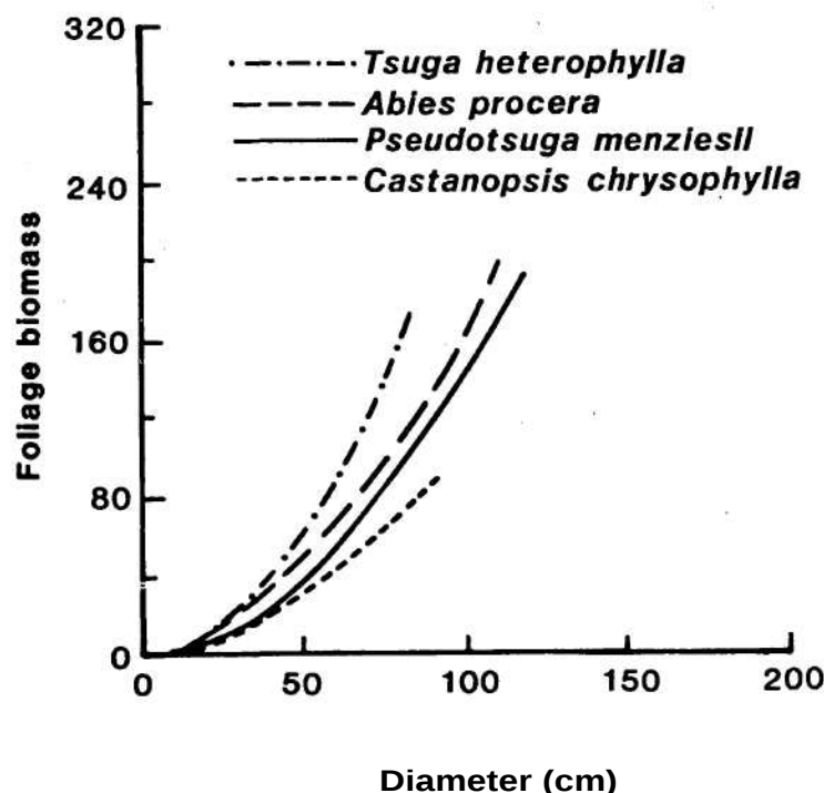
Figure 4.— Foliage biomass as related to diameter using the equations of Gholz and others (1979). A warning is given by Gholz and others (1979) that "maximum and minimum values from the data set...do not necessarily mean that the equation provides reasonable numbers at these extremes." Because of problems in exceeding the data ranges, the foliage biomass-d.b.h. relationship was modified using figure 5, as described in the text.
