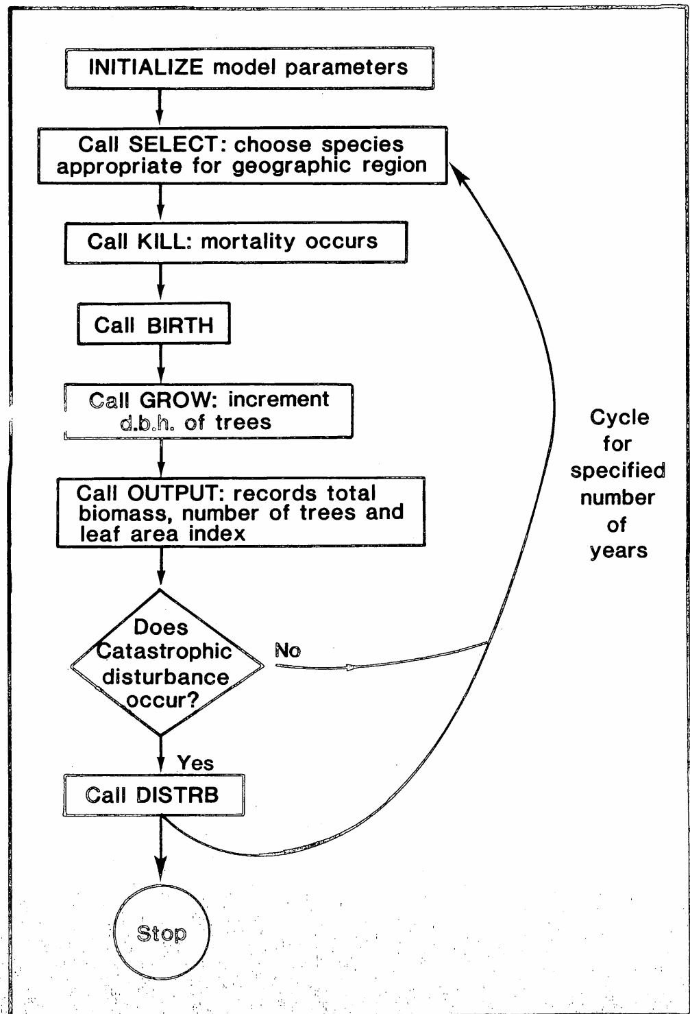
Figure 2.—General scheme of model.
