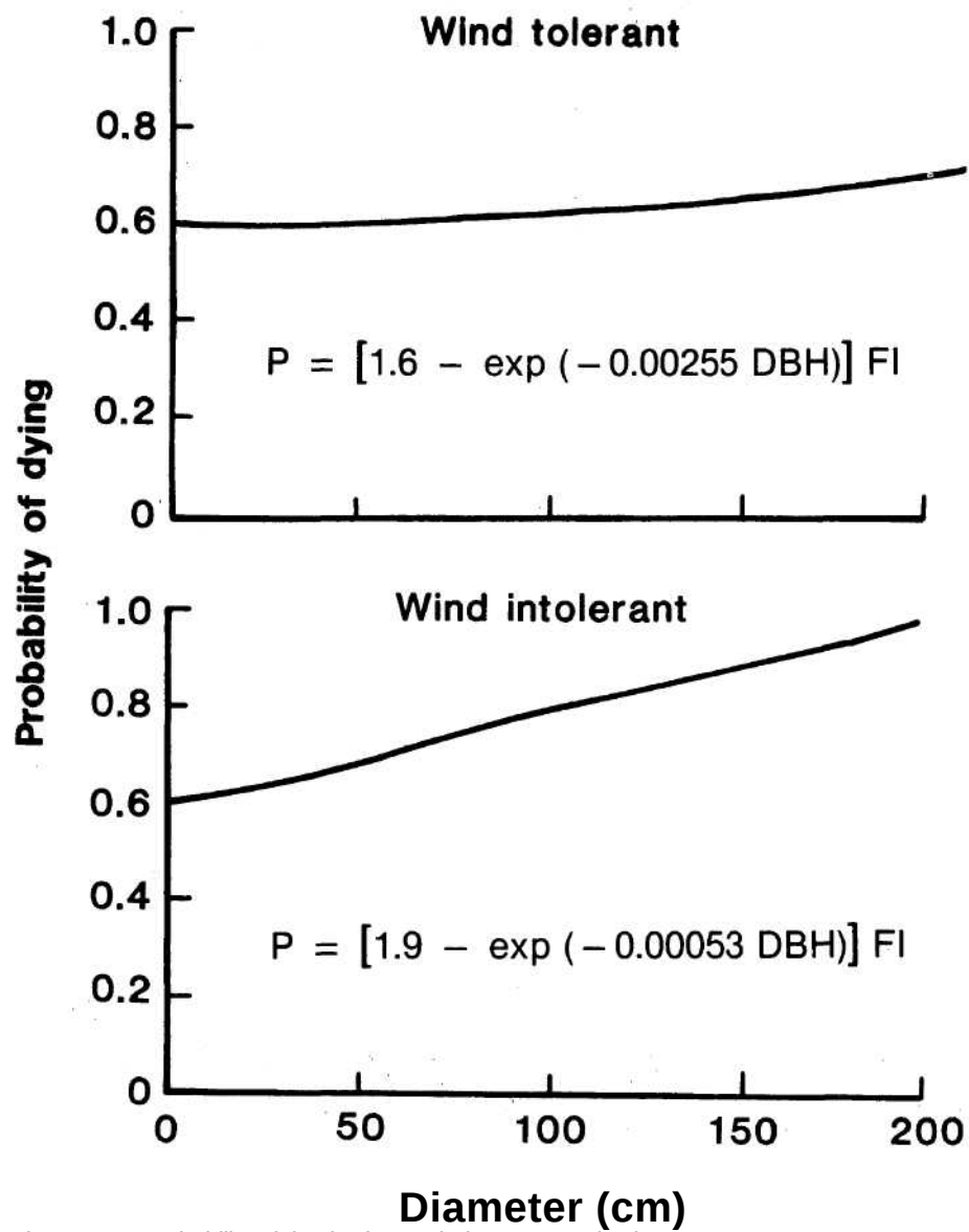
Figure 15.—Probability of death after a windstorm. Species in each tolerance class are listed in the text. The most severe storm is illustrated (FI = 1).
