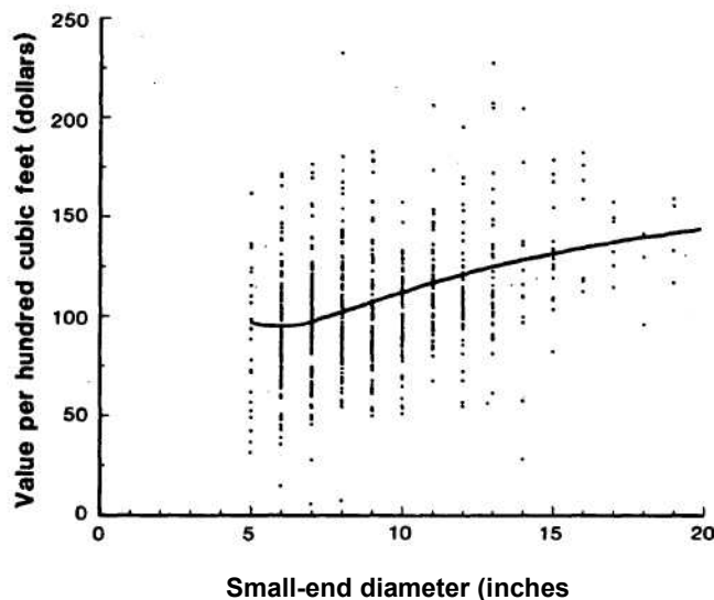
Figure 5.—Dollars per hundred cubic feet ($/CCF), by scaling diameter, for data combined from both mills. Cubic recovery percent and the average value of the lumber both increased with diameter; consequently, the $/CCF follows the same trend:
