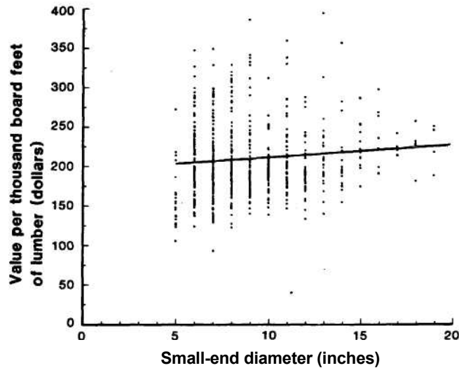
Figure 4.—Dollars per thousand board feet ($/MLT) of lumber tally, by scaling diameter, for both mills. This curve follows the general trend expected—value increasing with diameter. The limited size of the trees in the Black Hills, however, precludes the high value often obtained from ponderosa pine in areas where larger trees are prevalent:
