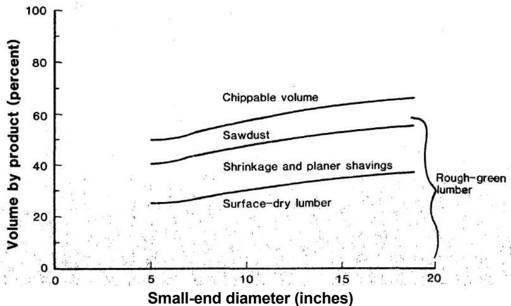
Figure 1—Volume of products, recovered expressed as a percentage of gross cubic foot volume of logs by diameter. This represents the combined recovery of mill-length logs from two sawmills, cutting 1-inch-thick lumber.
