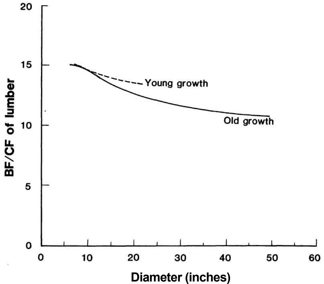
Figure 4.—The BF/CF ratio of lumber decreases as log size increases because
