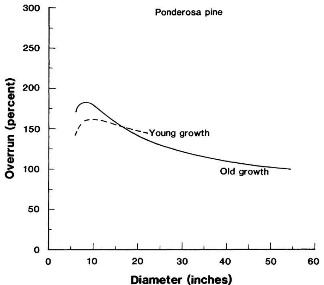
Figure 3—Scribner overrun decreases as log size increases because of the combined effects of log scale, taper, and product mix. Within the 6- to 16-inch range the overrun for young-growth logs is lower than the overrun for old-growth logs.
