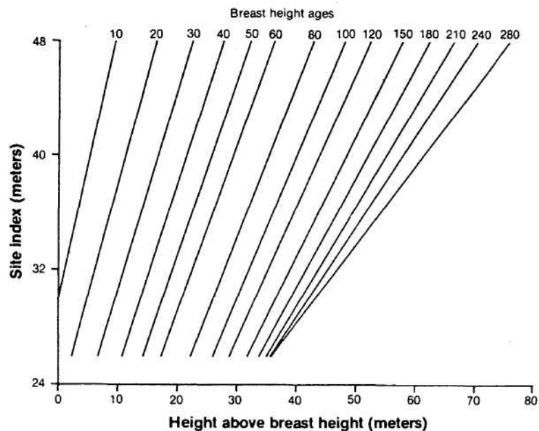
Figure 3.—Final site index estimating curves, equation (14), presented with the dependent variable (site index) on the vertical axis.
