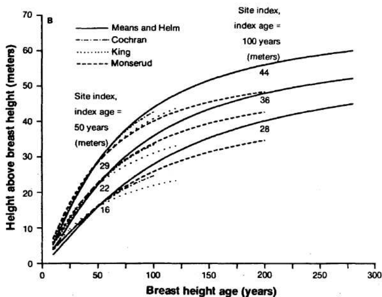
Figure 6.—Comparison of our height growth curves, equation (6), with height growth curves previously published for Douglas-fir. Site indices for these curves were chosen so they would cross our curves at their index ages: A, comparison of our curves with those of Curtis and others (1974b) and McArdle and others (1961); B, comparison of our curves with those of Cochran (1979), King (1966), and Monserud (1984).
