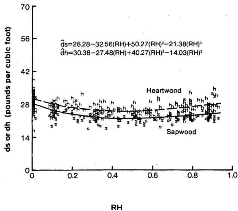
Figure 10.—Owendry sapwood and heartwood density profiles of Douglas-fir based on disk samples where: \hat{d}s = predicted owendry sapwood density, \hat{d}h = predicted owendry heartwood density, and RH = relative height (height to sampling point divided by total height of tree bole above a 1-foot stump).
