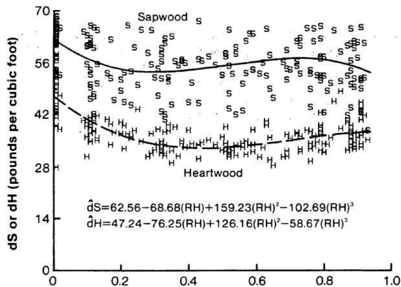
Figure 8.—Green sapwood and heartwood density profiles of Douglas-fir based on disk samples where: dS = predicted green sapwood density, dH = predicted green heartwood density, and RH = relative height (height to sampling point divided by total height of tree bole above a 1-foot stump).
