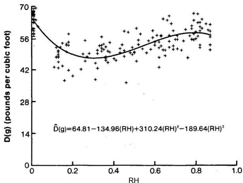
Figure 1a.—Greeji wood density profile of western hemlock based on disk samples where: D(g) = predicted green wood density, and RH = relative height (height to sampling point divided by total height of tree bole above a 1-foot stump).
