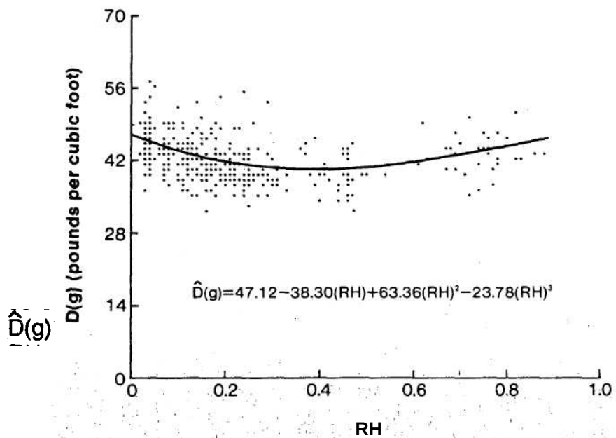
Figure 2b—Green Wood density profile of Douglas-fir based on core samples where: \hat{D}(g) = predicted green wood density, and RH = relative height (height to sampling point divided by total height of tree bole above a 1-foot stump).
