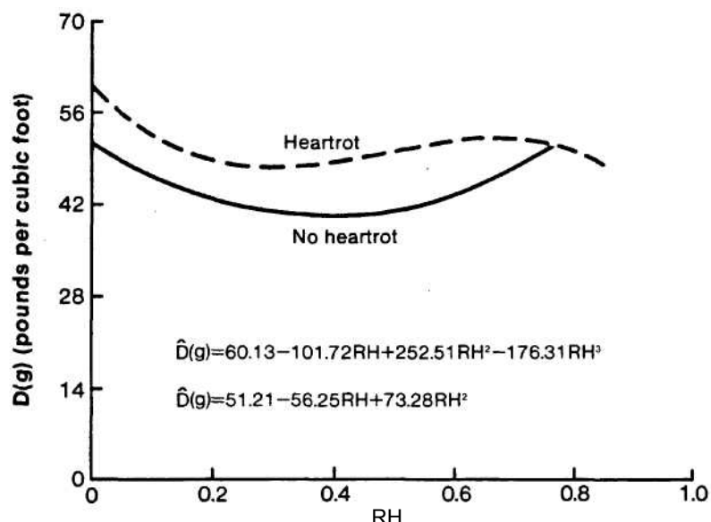
Figure 13.—Green wood density profiles of western hemlock for trees with and without heartrot. D(g) = predicted green wood density, and RH = relative height (height to sampling point divided by total height of tree bole above a 1-foot stump).
