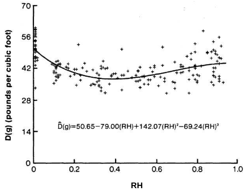
Figure 2a.—Green wood density profile of Douglas-fir based on core samples where: D(g) = predicted green wood density, and RH = relative height (height to sampling point divided by total height of tree bole above a 1-foot stump).
