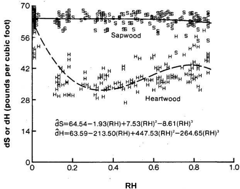
Figure 7—Green sapwood and heartwood density profiles of western hemlock based on disk samples where: dS = predicted green sapwood density, dH = predicted green heartwood density, and RH = relative height (height to sampling point divided by total height of tree bole above a 1-foot stump).
