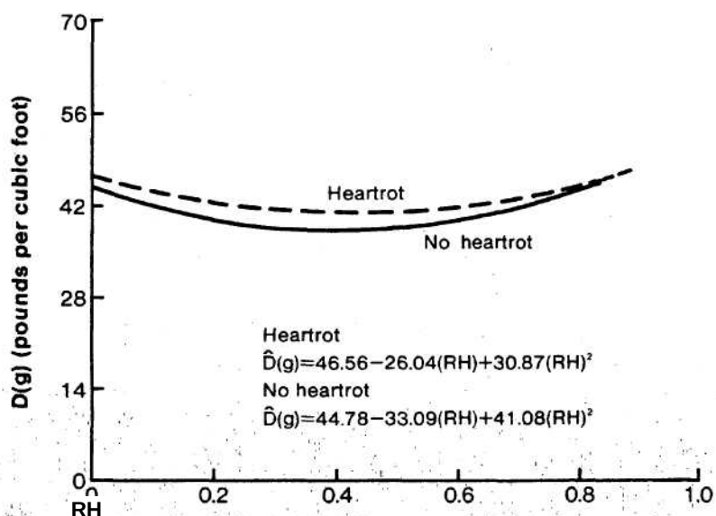
Figure 14.—Green wood density profiles of DouglasVfir for trees with and without heartrot. D(g) = predicted green wood density, and RH = relative height (height to sampling point divided by total height of tree bole above a 1-foot stump)
