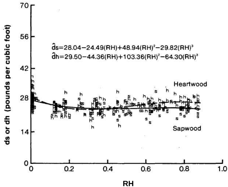
Figure 9.—Owendry sapwood and heartwood density profiles of western hemlock based on disk samples where: \hat{d}s = predicted owendry sapwood density, \hat{d}h = predicted owendry heartwood density, and RH = relative height (height to sampling point divided by total height of tree bole above a 1-foot stump).
