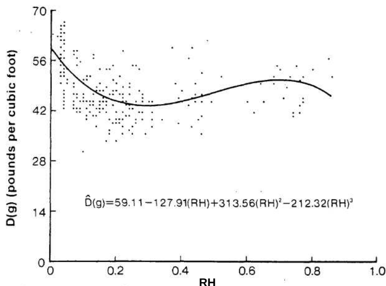
Figure 1b.—Green wood density profile of western hemlock based on core samples where: D(g) = predicted green wood density, and RH = relative height; height to sampling point divided by total height of tree bole above a 1-foot stump.
