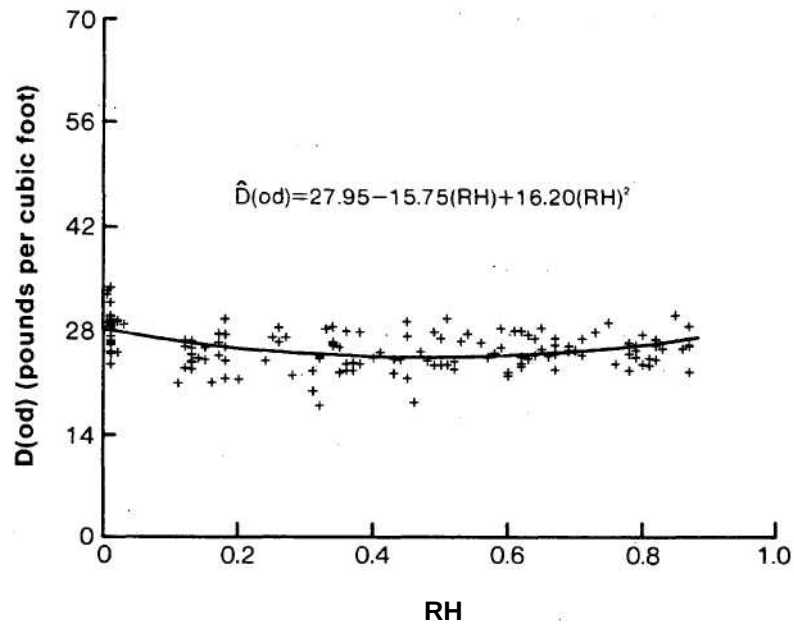
Figure 5.—Ovendry wood density profiles of western hemlock biased on disk samples where:
