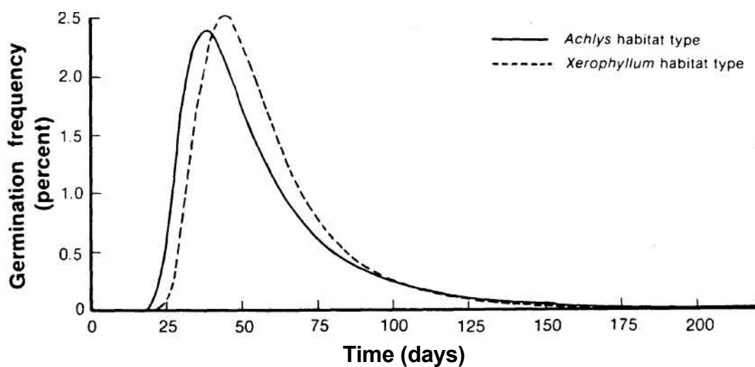
Figure 5.—Germination frequency in an unheated greenhouse of noble fir seeds on soils from Abies amabilis / Achlys and Abies amabilis / Xerophyllum habitat types.
