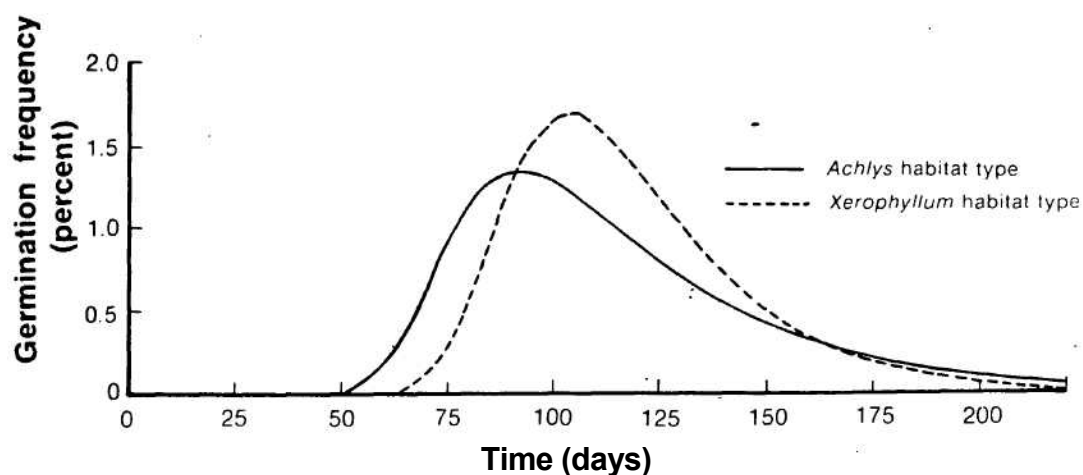
Figure 4.—Germination frequency in an unheated greenhouse of Douglas-fir seeds on soils from Abies amabilis / Achlys and Abies amabilis / Xerophyllum habitat types.
