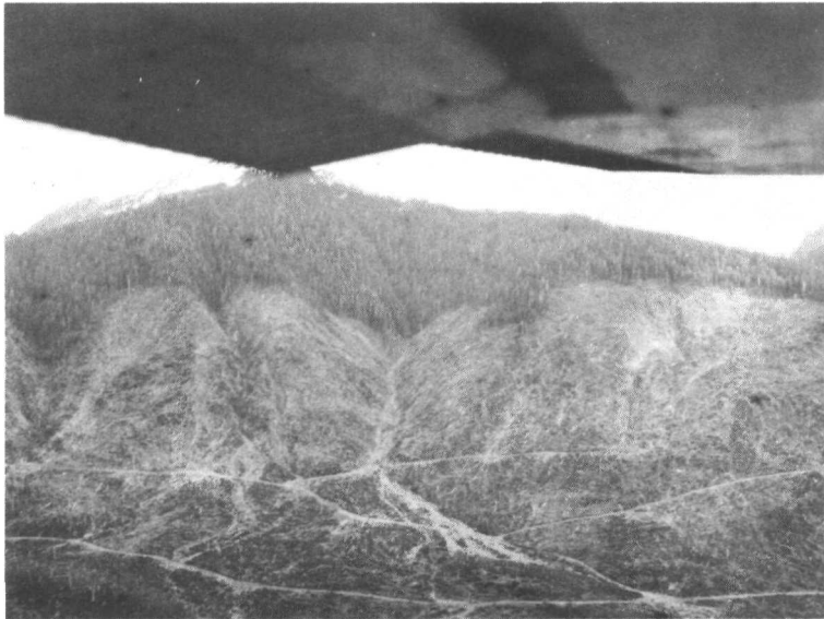
Figure 3-a. Three debris torrents in the Maybeso Creek valley. Prince of Wales Island, Alaska. All three developed during a high-intensity storm in the fall of 1961. Initial failure occurred at debris dams near the upper limit of logging in all three ravines.
