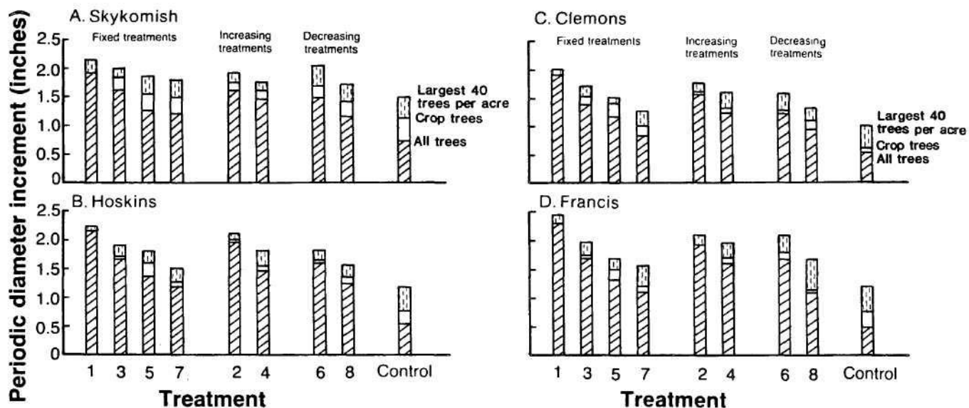
Figure 31.—Periodic diameter increment of the largest 40 trees per acre, crop trees, and all surviving trees, for fourth treatment period: (A) Skykomish, (B) Hoskins, (C) Clemons, and (D) Francis.
