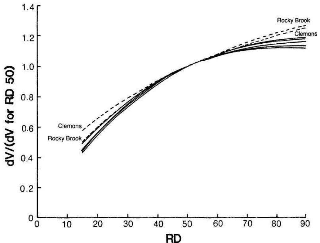
Figure 25.—Comparison of shapes of installation curves ( \ln dV = a_1 + b \ln RD + cRD + d \ln(H_i/H_m) ) fitted with common slopes for periods within a single installation. Estimates expressed as ratios of estimated dV to expected dV for RD50.
