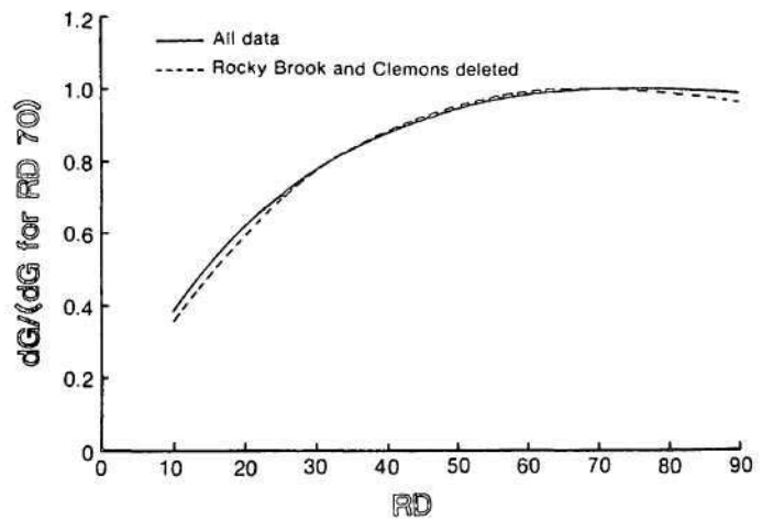
Figure 22.—Ratio of estimated dG to expected dG for RD70, based on the regression (\ln dG = a_i + b \ln RD + c RD) fitted to combined data under the assumption of common b and c coefficients for all installations and periods.
