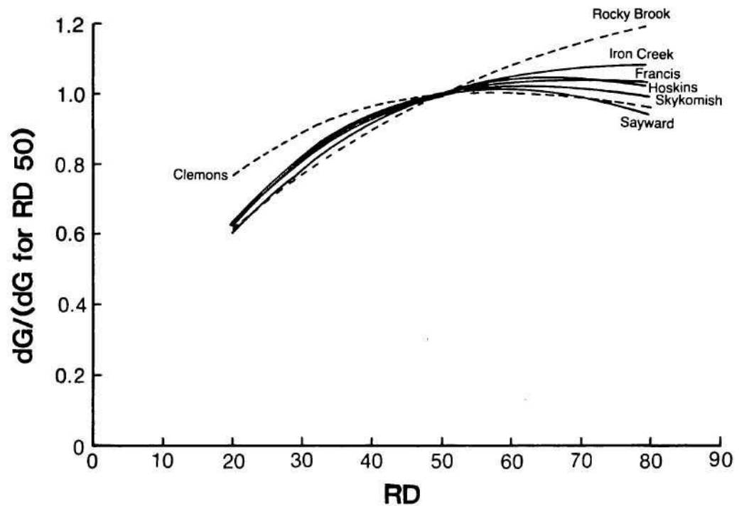
Figure 21.—Comparison of shapes of installation curves ( \ln dG = a; + b \ln RD + cRD ) fitted with common slopes for all periods within a single installation. Estimates expressed as ratios of estimated dG to expected dG for RD50.
