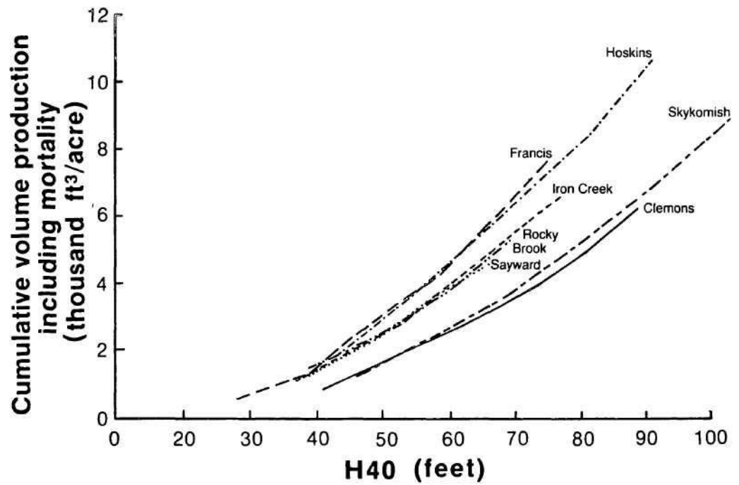
Figure 12.—Cumulative gross volume production in relation to H40 for control plots, by installation, all species.
