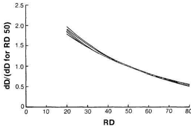
Figure 28.—Comparison of shapes of installation curves ( \text{IndD} = a + b\text{RD} + c\ln(\text{Hi}/\text{Hm}) ) fitted with common slopes for all periods within a single installation. Estimates expressed as ratios of estimated dD to expected dD for RD50.
