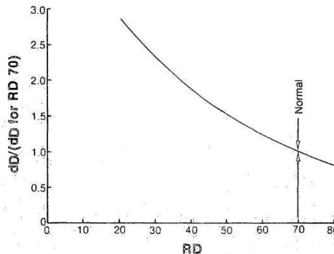
Figure 29.—Ratio of estimated periodic annual increment in diameter: (dD) to expected dD for RD70, based on the regression ( \text{IndD} = a + b\text{RD} + c\ln(\text{Hi}/\text{Hm}) ) fitted to combined, data assuming common slopes for all installations and periods.
