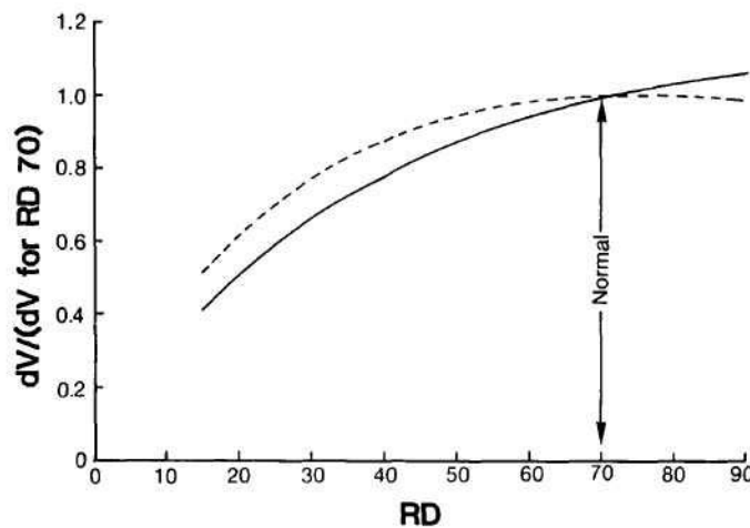
Figure 26.—Ratio of estimated periodic annual increment in gross volume (dV) to dV expected for RD70, based on the regression ( \text{IndV} = a + b \ln \text{RD} + c \text{RD} + d \ln(\text{Hi}/\text{Hm}) ) fitted to combined data, assuming common slopes for all installations and periods. Dashed line represents similar curve for gross basal area increment.
