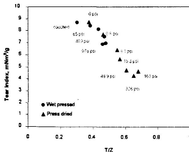
Figure 1. Tear index at various levels of bonding (Tensile index / Zero span tensile index) of TMP (110 CSF) wet pressed and press dried to various levels of bonding
