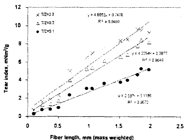
Figure 4. Fiber length dependency in the low bond strength region
