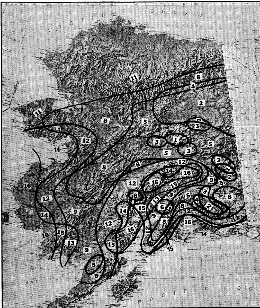
Figure 4.—Map showing composite PEI-TEI climatic zones produced when map in figure 2 is overlaid on that of figure 3.
