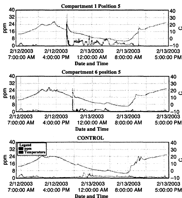
Figure 5. Real-time Langan CO measurements at positions 1–5 (Plot 1), 6–5 (Plot 6) and the check location.
