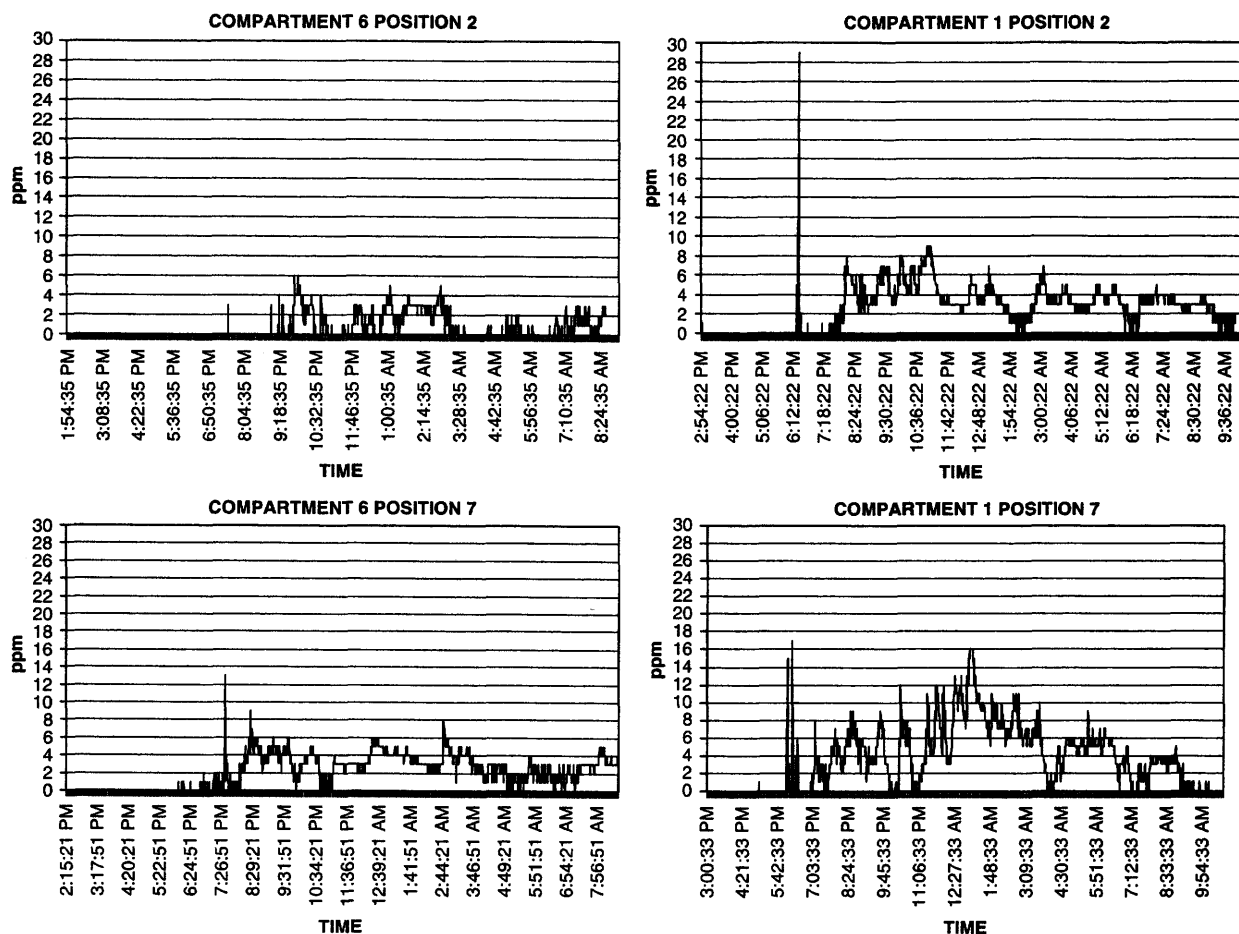
Figure 6. Real-time draeger CO measurements at positions 6–2 and 6–7 in the chipped plot and positions 1–2 and 1–7 in the non-chipped plot.
