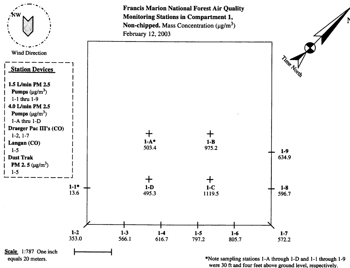
Figure 3. Time-integrated PM 2.5 measurements at interior and perimeter sampling locations in compartment 1 (Non-Chipped Plot).
