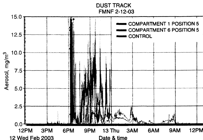
Figure 4. Real-time DustTrak PM 2.5 measurements at positions 1–5 (Plot 1), 6–5 (Plot 6) and the check location.
