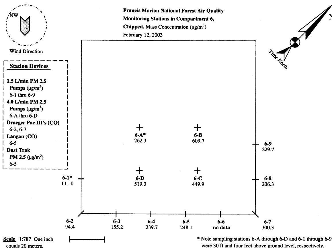
Figure 2. Time-integrated PM 2.5 measurements at interior and perimeter Sampling locations in compartment 6 (Chipped Plot).
