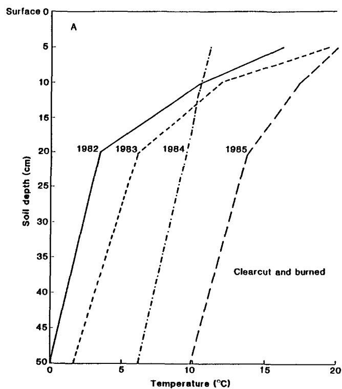
Figure 4—A. Soil temperature profile in mid-July at a clearcut and burned plot (11) before logging (1982) and the first 3 years after treatment (1983-85).
