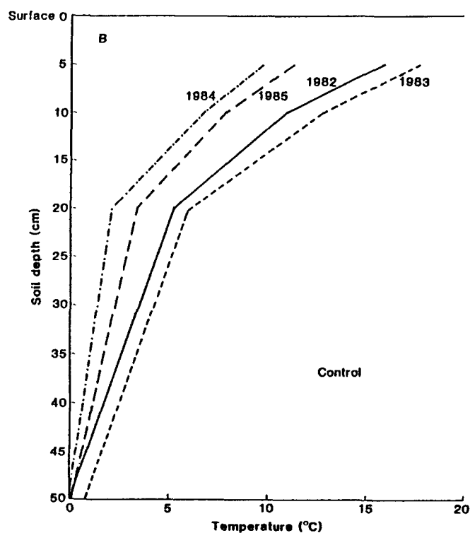
Figure 4—B. Soil temperature profile in mid-July on a paired, undisturbed control plot (12) for 1982-85.
