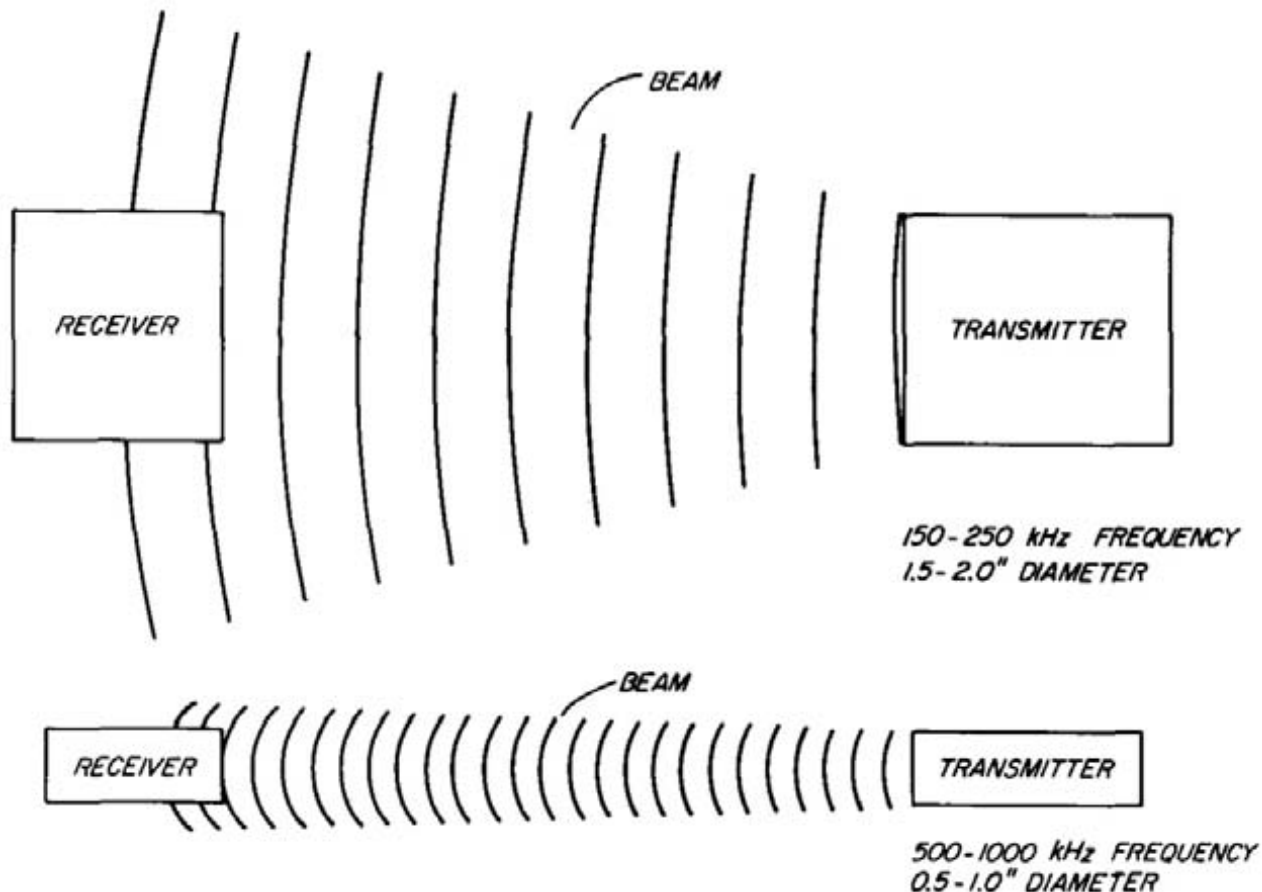
Figure 5.—Upper: The wide beam of sound is a result of the low transmitted frequency (150 to 250 kHz) and means poor resolution of a defect area.
