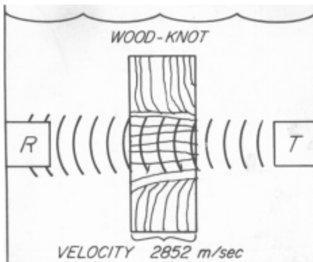
Figure 9.-Velocity and received waveforms of sound propagated through water alone, through clear wood, and through a knot.
