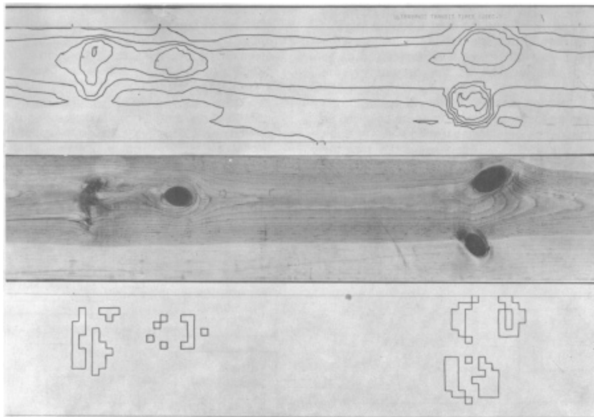
Figure 13.—Upper: Contour plot of ultrasonic transit time data, showing the close correlation to the grain pattern of this pine board.
