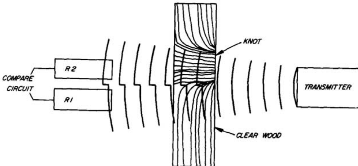
Figure 16.—Two transducers are used to receive the transmitted sound pulse for comparison of the sound velocity through wood at two points.
