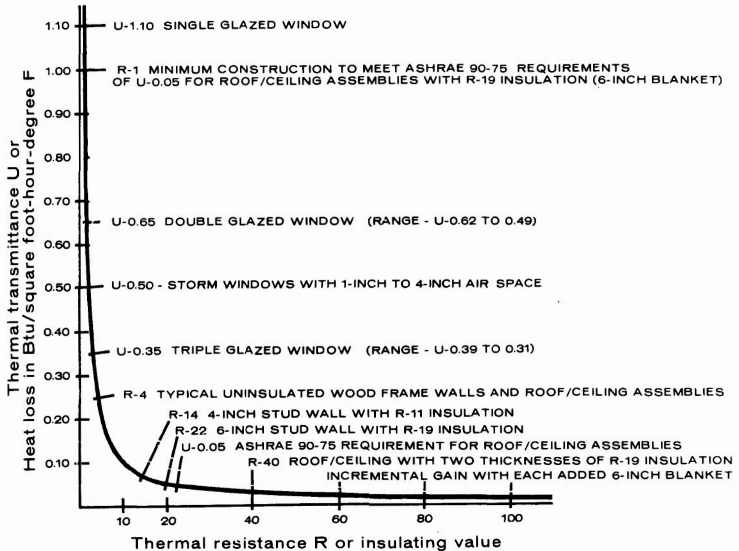
Figure 5.—Plot of thermal transmittance ( U ) against thermal resistance ( R ); at U values below 0.10, increases in efficiency become increasingly expensive.
