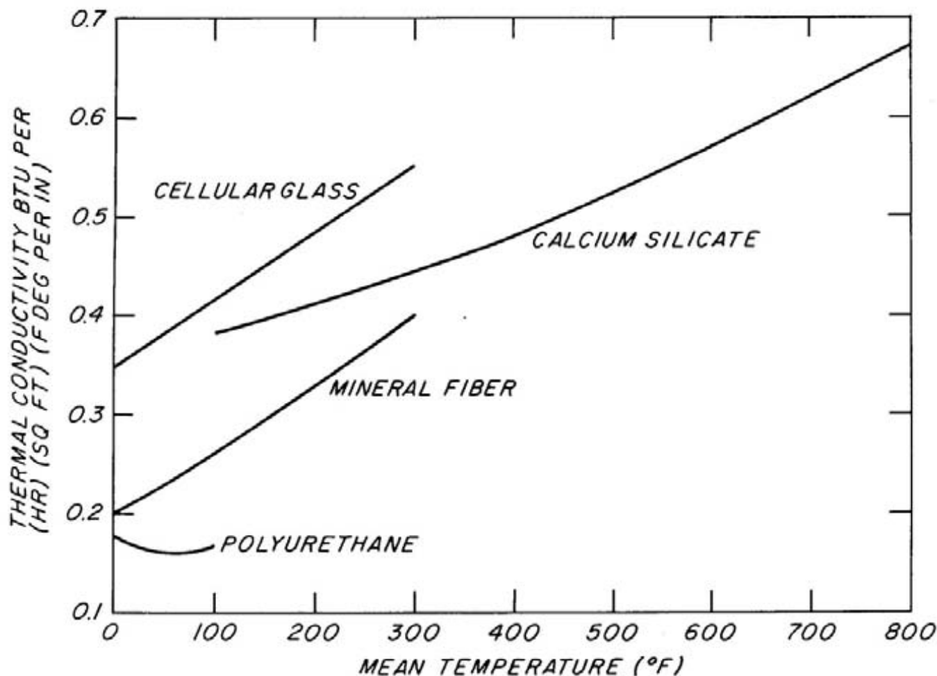
Figure 7.—Typical variation of thermal conductivity with mean temperature (ASHRAE Handbook, 1977). (M 146 477)
