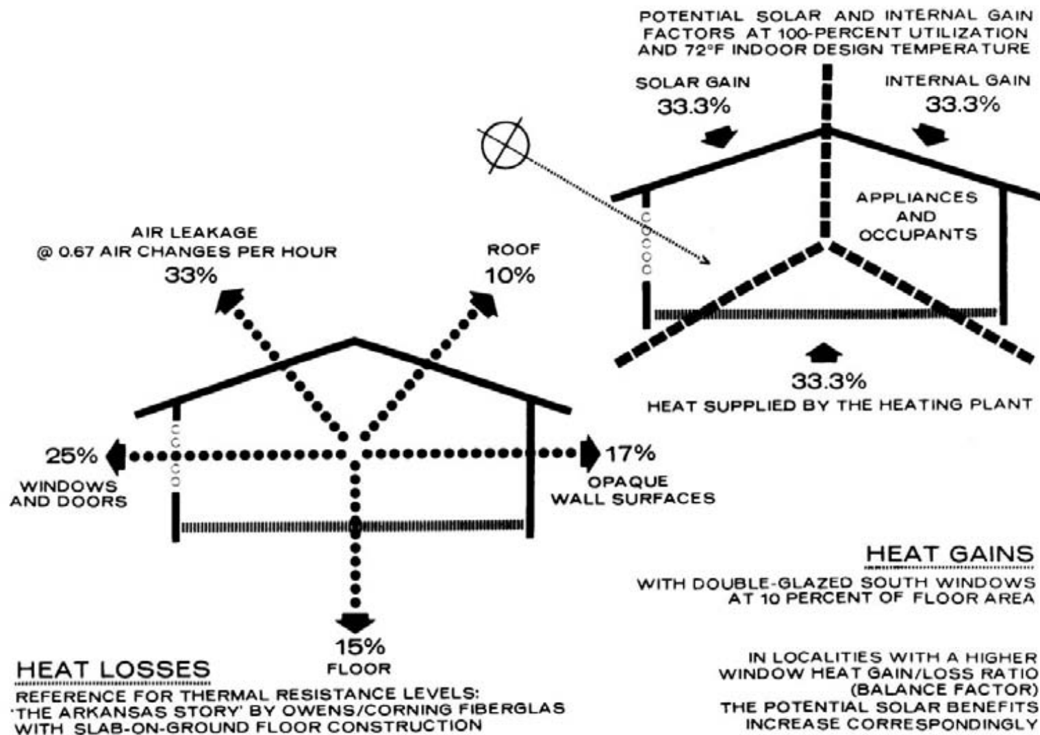
Figure 1 .-Heating season energy balance for a 6 Btu/sq.ft.-degree day house at Madison, Wisconsin conditions.
