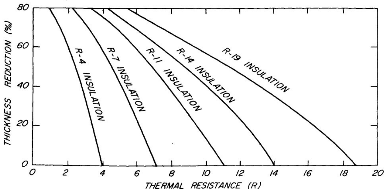
Figure 10.—Reduction in thermal resistance of fibrous insulation due to compression to reduce thickness. (From HUD Mobile Homes Federal Construction and Safety Standards, 1976).
