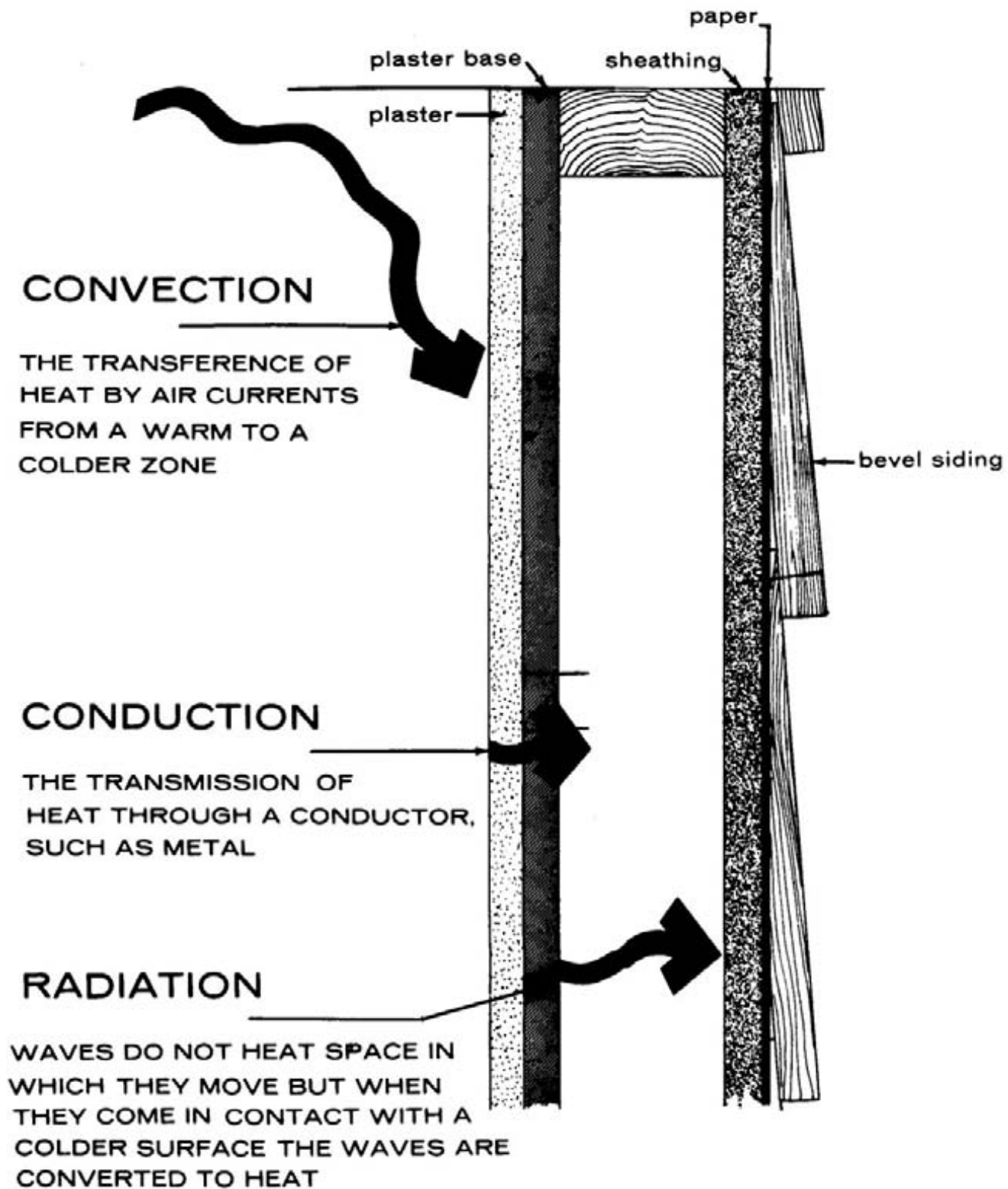
Figure 6.—Modes of heat transfer in light-frame wall.
